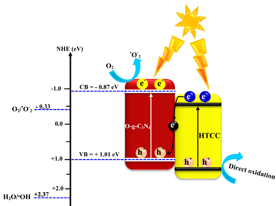
Fig. 7. The possible Z-scheme mechanism proposed for the \text{O-g-C}_3\text{N}_4/\text{HTCC} photocatalyst (The modified form with permission from reference [13] 2019 Elsevier).
