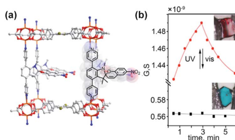
Fig. 24 (a) Single crystal X-ray structure with simulated spiroyrans pillars showing isomerization to merocyanine form. (b) Light-induced changes in the conductance of the single crystal of the MOF bearing spiroyrans pillars (red line) and control non-responsive MOF (black line). Adapted with permission from ref. 146. Copyright 2019 American Chemical Society.
