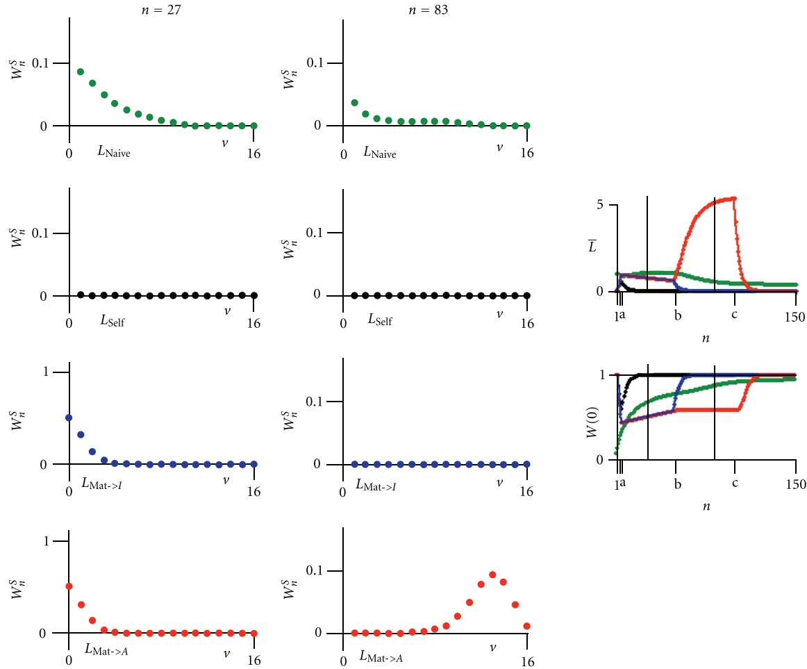
FIGURE 13: Computer result of the maturation process of T-lymphocytes. First a naïve T-lymphocyte ( L_{Naive} , green) in bone marrow or thymus undergoes T-cell receptor rearrangement ( \beta -selection). T-cells with high affinity to self-peptides MHC ( L_{Self} , black) are eliminated (negative selection), whereas T-cells with T cell receptors that are able to bind self-peptides MHC molecules with at least a weak affinity ( L_{Mat->I} , blue and L_{Mat->A} , red) survive (positive selection) and circulate in the peripheral lymphatic system. The matured T-lymphocyte, recognizing the antigen by high affinity to the antigen-loaded MHC ( L_{Mat->A} , red), transforms into an effector cell and proliferates. Glimpses at generation at n = 27 and n = 83 . Left: probabilities W_n^S(N) of finding N individuals of T lymphocytes ( 0 \leq N \leq N_{max} ). Upper right: extinction probability W(0) as a function of generations n . Lower right: average of T lymphocytes \bar{L} as a function of generations n . Parameter values and their change during the dynamics (a) n < 50 (b) 50 \leq n < 100 (c) 100 \leq n : maximal total number N_{max} = 16 ; \alpha_{L_{Naive}} = 0.1 , \alpha_{L_{Self}} = 0.1 , \alpha_{L_{Mat->I}} = 0.1 , \alpha_{L_{Mat->A}} = 0.1 , \rho_{L_{Naive}} = 2 , \rho_{L_{Self}} = 1 , \rho_{L_{Mat->I}} = 1 , \rho_{L_{Mat->A}} = 1/4/1 , \beta_{L_{Naive}} = 0.95 , \beta_{L_{Self}} = 0.75 , \beta_{L_{Mat->I}} = 0.99/0.75/0.75 , \beta_{L_{Mat->A}} = 0.99/0.98/0.75 , \varepsilon_{L_{Naive}L_{Self}} = 0.7 , \varepsilon_{L_{Naive}L_{Mat->I}} = 0.7 , \varepsilon_{L_{Naive}L_{Mat->A}} = 0.7 .
