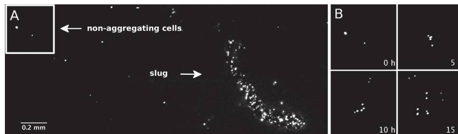
Figure 5. Non-aggregating cells grow on new incoming nutrients. 18h after plating cells on nutrient-free agar, aggregating cells have formed slugs while non-aggregating cells are starving. Fresh nutrients (dead bacteria) were added at this point. A ) Red fluorescence image of slugs and non-aggregating cells at the time of new nutrient supply. B ) Inset from A showing a non-aggregating cell that resumes dividing over time upon addition of new nutrients (the number of red dots increases over time as non-aggregating cells divide). Non-aggregating cells are capable of resuming growth immediately upon food arrival while aggregating cells are embedded in development.
