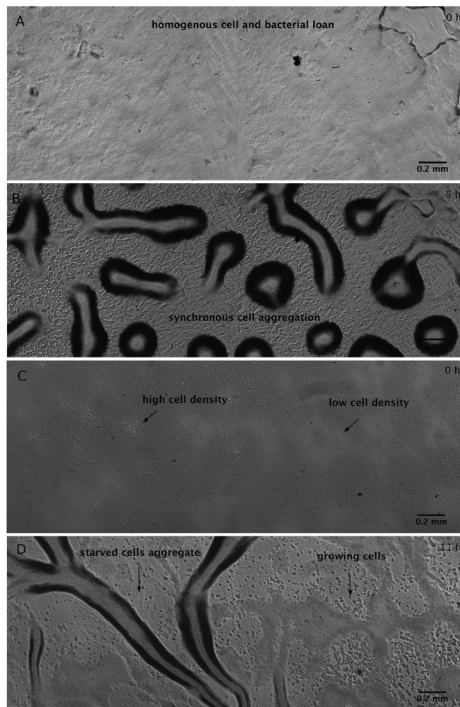
Figure S3. Cell aggregation on homogenous or heterogeneous bacterial lawns. AX3 cells were plated mixed with bacterial suspensions and plated on nutrient-free agar either homogeneously (A) or heterogeneously (C). Homogeneous plating yields a synchronous timing of starvation and aggregation over the whole plate (B). Heterogeneous plating yields a non-uniform timing of starvation and aggregation, with aggregates forming in some areas while cells are growing in other areas (D) of the same plate.
