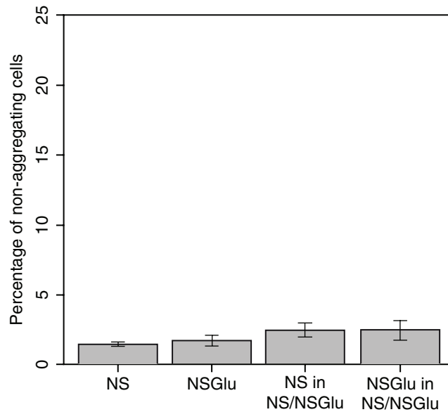
Figure S4. Effect of NS and NS Glu medium on non-aggregating cell fractions. Cells were grown either on NS and NS with 85mM glucose (NS Glu) medium. Cells grown on either medium show no differences with respect to the non-aggregating cell fraction when alone compared to when NS-grown and NSGlu-grown cells are mixed together. Error bars represent +/- standard deviation ( 6 \leq n \leq 8 ). A one-way ANOVA test yielded F=1.54 , p=0.27 .
