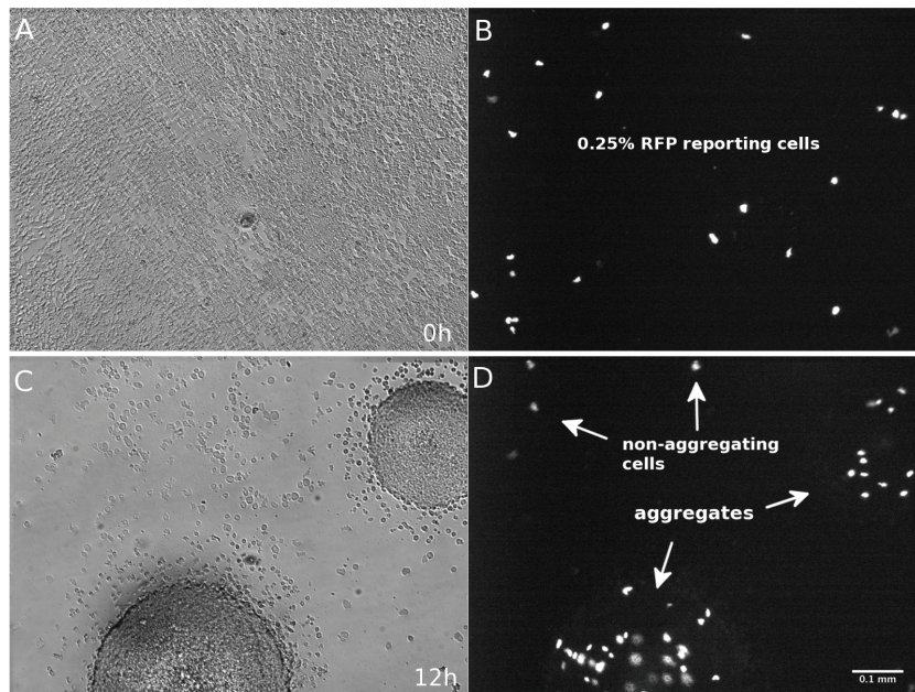
Figure 1. Upon starvation, a D. discoideum population partitions into aggregating and non-aggregating cells. AX3 cells were plated on nutrient free-agar and imaged before ( A, B ) and after ( C, D ) aggregation. A and C are phase contrast images, B and D are red fluorescence images. In B and D , 0.25% of AX3 RFP cells appear as single dots within a population of AX3 GFP cells. The percentage of non-aggregating cells was estimated as the ratio of dots counted outside aggregates after aggregation and dots counted before aggregation.
