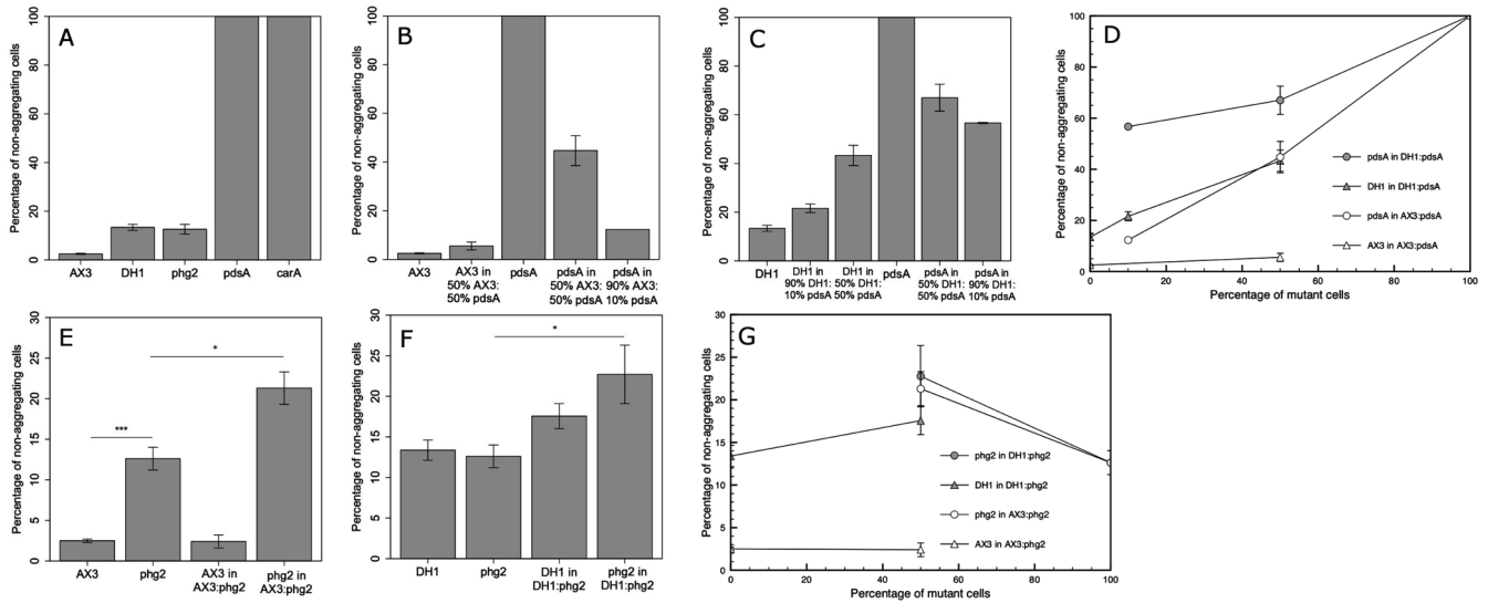
Figure 3. Genetic factors affect population partitioning. The percentage of non-aggregated cells (at initial density 3 \times 10^6 cells/cm 2 ) was measured for genetically different wild-type strains (AX3 and DH1) and single-gene mutants ( phg2 , pdsA , carA ) alone (A), and in mixtures between wild-type and single-gene mutant strains: mixtures of pdsA with AX3 (B) or DH1 (C), and mixtures of phg2 with AX3 (E) or DH1 (F), varying the percentage of mutant cells in mixtures. Wild-type DH1 cells aggregate less than wild-type AX3 cells (A). phg2 mutant cells aggregate as well as their parent DH1 strain cells, while pdsA and carA cells do not aggregate on their own (A). The presence of AX3 or DH1 cells rescues pdsA cell aggregation (B–D). In turn, DH1 cells aggregate less than on their own when increasing the percentage of pdsA cells in DH1: pdsA mixtures, while AX3 cells aggregate as well as on their own in the presence of AX3 or DH1 cells. DH1 cells aggregate less than on their own in DH1: phg2 mixtures, while AX3 cells aggregate as well as on their own in the presence of phg2 cells (E–G). The non-aggregating cell fraction of the global mixed DH1: phg2 or AX3: phg2 population is higher than that of either pure populations, respectively DH1 and phg2 , or AX3 and phg2 . Overall, cell genotype determines the fraction of aggregating cells, and cells of different genotypes affect each other's non-aggregating cell fraction in mixtures. Error bars represent \pm standard deviation. * represents p < 0.05 ( 2 \leq n \leq 9 ). *** represents p < 0.001 (horizontal bars indicate the corresponding pairs of statistical samples).
