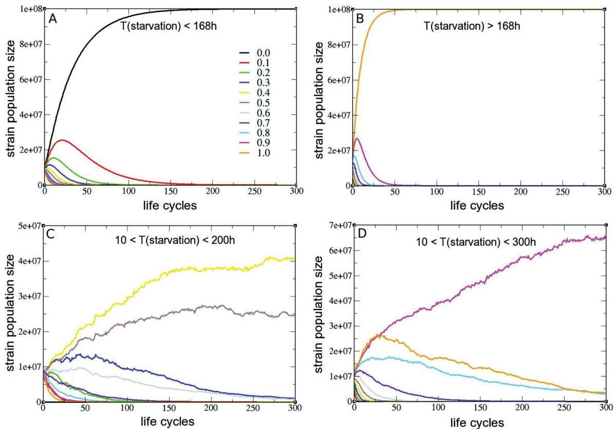
Figure 6. Population partitioning is advantageous in fluctuating environments. Our numerical model involves eleven strains with different fixed investments into non-aggregating cells that were competed under different starvation conditions. Strain investment into non-aggregating cells varies from 0 to 1, with 1 corresponding to complete aggregation and 0 to no aggregation. The duration of the starvation period was varied from <168\text{h} (A), >168\text{h} (B), randomly taken between 10h and 200h (C), randomly taken between 10h and 300h (D). For systematically long ( >168\text{h} , B) and short ( <168\text{h} , A) durations of starvation, strains with 100% aggregation and 0% aggregation take over respectively. For random starvation duration, a particular aggregation rate is selected, for instance 0.4 for 10\text{h} < T < 200\text{h} (C) and 0.9 for 10\text{h} < T < 300\text{h} (D), and thus the superimposition of both strategies is the optimal response.
