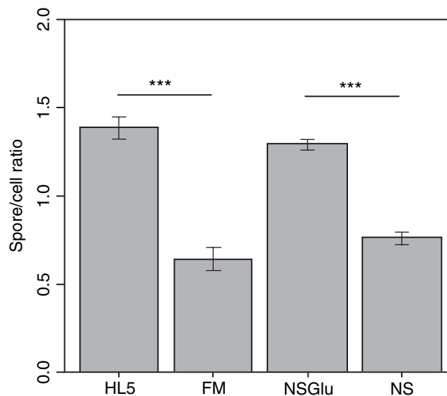
Figure S5. Nutritional state of the cells biases spore/stalk differentiation in aggregates. RFP-expressing AX3 and GFP-expressing AX3 cells were grown on one of 4 different media: HL5 (rich medium), FM (minimal medium), NS Glu (rich medium with glucose) and NS (rich medium without glucose). Cells grown on these media were mixed at 1:1 ratio for HL5:FM and NSGlu:NS mixtures. The ratio of spore percentage over plated cell percentage of each cell population in the 1:1 mixture indicates if one population is getting enriched into spores with respect to the other one. For spore/cells ratios = 1 both populations contribute equally to spores. If spore/cells ratio > 1, the population is enriched in spores, and if spore/cells ratio < 1, the population is underrepresented in the spores. We find that HL5-grown cells are over-represented in the spores in mixture with FM-grown-cells, FM-grown cells are underrepresented in the spores in mixture with HL5-grown cells. We confirm previously published data showing that NSGlu-grown cells are over-represented in mixture with NS-grown-cells, NS-grown cells are underrepresented in the spores in mixture with NSGlu-grown cells. Error bars represent +/- standard deviation ( 11 \leq n \leq 18 ). *** represents p < 0.001 (horizontal bars indicate the corresponding pairs of statistical samples).
