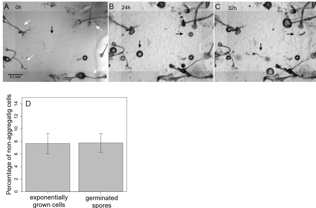
Figure 4. Cells switch between aggregating and non-aggregating fates. A–C Non-aggregating cells have not stably lost the ability to aggregate. A ) After the completion of aggregation and formation of fruiting bodies (white arrows), bacteria were added to areas with non-aggregating cells (black arrows). Non-aggregating cells grow and divide on fresh nutrients (see Figure 5). Once bacteria are consumed, the descendants of non-aggregating cells aggregate (B) and develop into a fruiting body (C) . D ) A population of germinated spores re-partitions into aggregating and non-aggregating cells upon starvation. A population of spores was germinated and grown on bacteria for 3–5 cell divisions. When this population is plated on a nutrient-free substrate it partitions into aggregating and non-aggregating cells with the same proportions as populations of exponentially growing cells submitted to starvation. Error bars represent \pm standard deviation ( 4 \leq n \leq 7 ).
