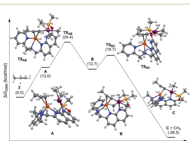
Fig. 5 Calculated energy profile for alkyne activation and DFT-optimized structures for intermediates and transition states.
