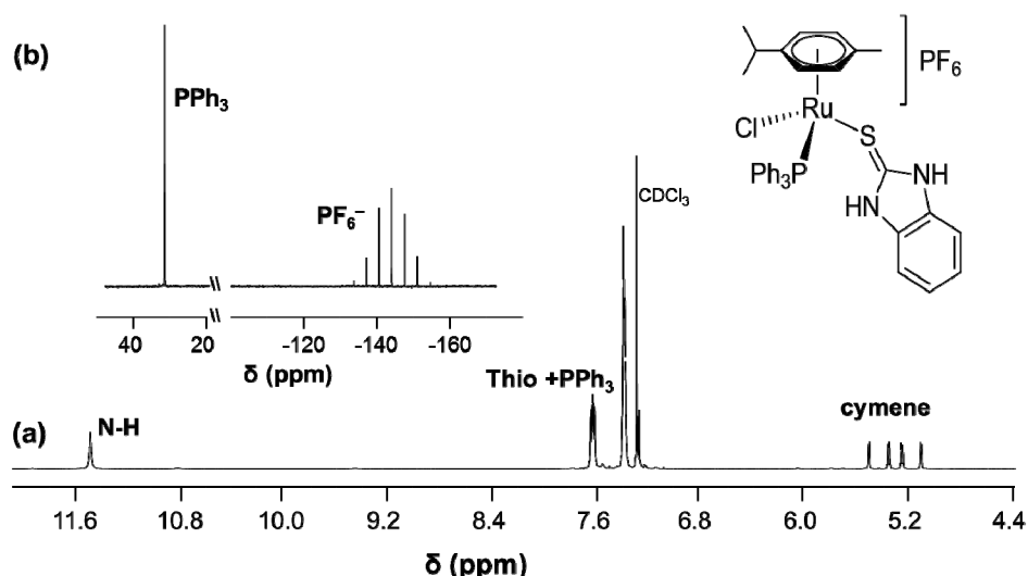
Figure 1. (a) The downfield region of the ^1\text{H} -NMR spectrum of 13 . (b) ^{31}\text{P}\{^1\text{H}\} -NMR spectrum showing a singlet at 29.5 ppm ( \text{PPh}_3 ) and a septet at -144.2 ppm ( \text{PF}_6^- ).
