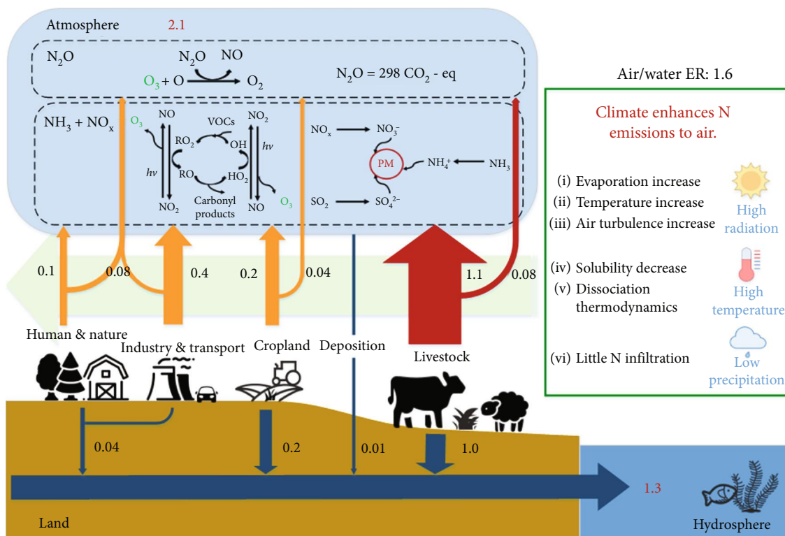
FIGURE 1: N_r emission to air as compared to water in Australia. ER: emission ratio. Units of these numbers are Tg N_r yr^{-1} . The green box indicates that climate in Australia enhances N emissions to air other than water. “Livestock” includes both grazing and feedlot emissions; “Deposition” includes both dry and wet N deposition to fresh surface water; “Cropland” includes both dryland and irrigated land emissions; “Industry & Transport” includes both industry and transport emissions; “Human & Nature” includes all emissions from human, aquaculture, forest, pets, urban green-land, and waste treatment sectors. Livestock is the largest emission source, with 1.2 Tg N_r release to the atmosphere per year and 1.0 Tg N_r emissions to the hydrosphere per year. Climate in Australia enhances N emissions to air other than to water. High solar radiation increases water evaporation, surface temperature, and air turbulence, all promoting N emissions to air; high temperature increases NH_3 volatilization rate because of its solubility and dissociation thermodynamics; low precipitation indicates little N infiltration, reducing N emissions to water.
