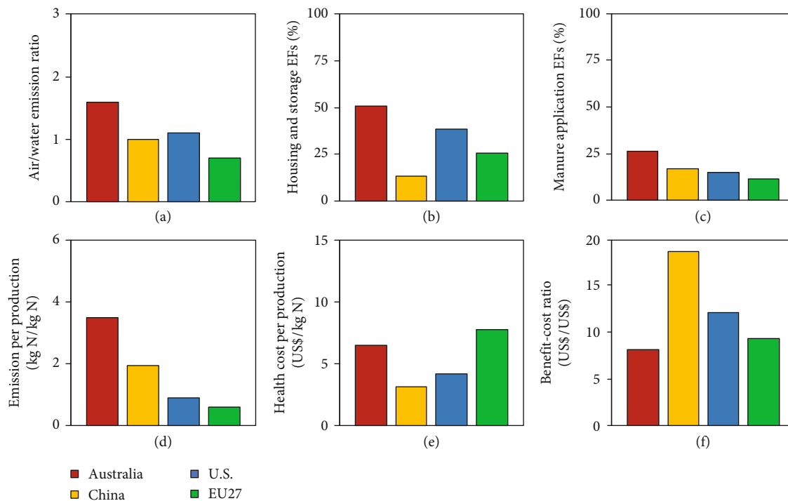
FIGURE 3: Comparison of N_r emission factors and associated cost and benefit between Australia and other countries: (a) air/water emission ratio; (b) livestock housing and manure storage \text{NH}_3 emission factors; (c) manure application \text{NH}_3 emission factors; (d) atmospheric emission per livestock production; (e) health cost per livestock production; (f) benefit-cost ratio of livestock industry (including feedlot and animal grazing). “Emission per production” represents the atmospheric N emission for each kg N accumulated in livestock products; “Health cost per production” indicates the health cost related to atmospheric N emission for each kg N accumulated in livestock products; “Benefit-cost ratio” is the ratio of income and total cost (including feed and health damage) in livestock industry.
