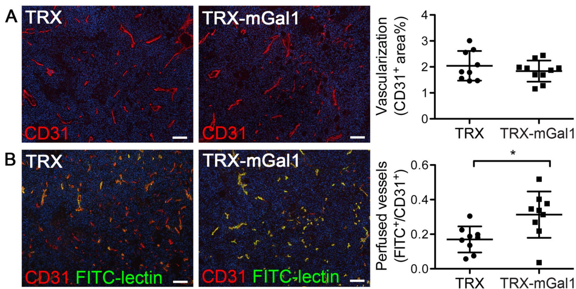
Fig. 3 Tumor vascular perfusion is improved after vaccination against Gal1. a Representative immunostaining for blood vessels (CD31, red) and quantification of CD31-positive area (% of 10 \times field). B FITC-LEL perfused blood vessels (green) and immunostaining for blood vessels (CD31, red). The proportion of FITC-LEL positive blood ves-
