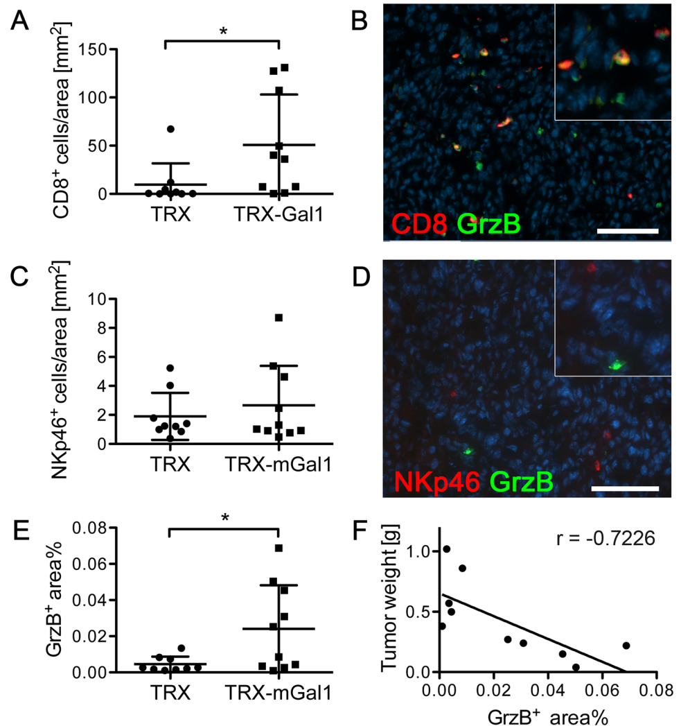
Fig. 6 Cytotoxic activity of CD8^+ T cells is increased in tumors from Gal1 immunized mice. a Quantification of CD8^+ cells per mm^2 in tumors from TRX (control) or TRX-mGal1 immunized mice ( p=0.0247 ). b Representative immunostaining for cytotoxic T cells (CD8, red) and granzyme B (GrzB, green). c Quantification of NKp46-positive cells per mm^2 ( p=0.9048 ). d Representative immunostaining of NK cells (NKp46, red) and granzyme B (GrzB, green). e Quantification of granzyme B (positive area % per 10X field; p=0.0373 ). f Correlation of GrzB-positive area (% of 10X field) and tumor weight in TRX-mGal1 immunized mice at termination of the experiment ( p=0.0182 , Pearson correlation coefficient r=-0.7226 ). Statistical differences between the groups were determined by Mann–Whitney U test (data not normally distributed). All graphs illustrate mean values \pm SD, and each dot represents an individual. Scale bars: 100 \mu m
