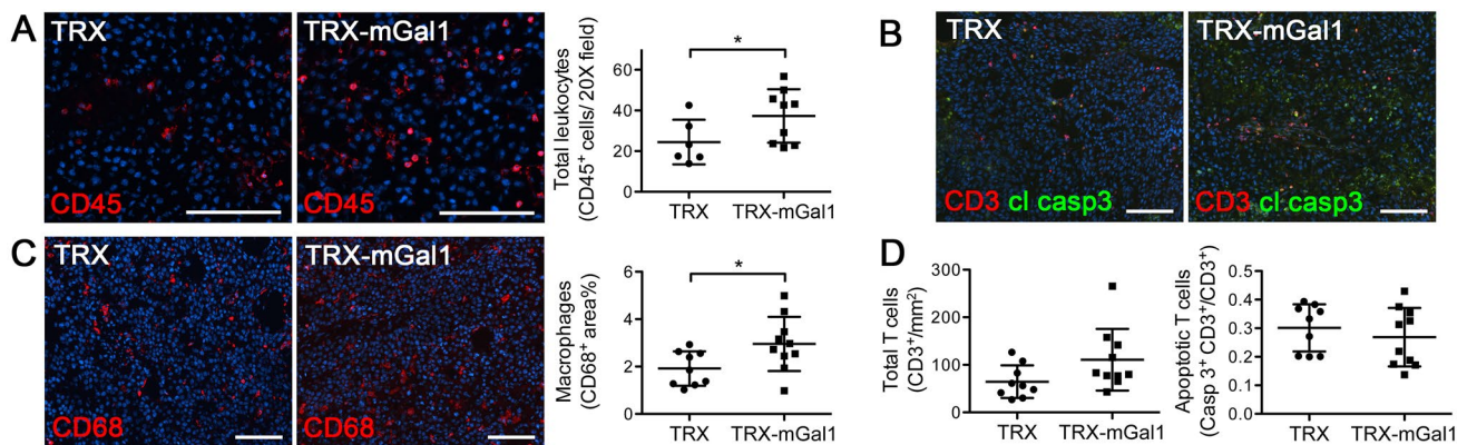
Fig. 4 Leukocyte recruitment to tumors is enhanced in Gal1 immunized mice. a Representative immunostaining for leukocytes (CD45, red) and quantification of CD45 + cells (per 20× field). The difference in CD45 + cell infiltration between the groups was assessed by Mann–Whitney U test (data not normally distributed), p=0.0496 . b Representative immunostaining for T cells (CD3, red) and apoptotic T cells by cleaved caspase-3 staining (green). c Representative immunostaining for macrophages (CD68, red) and quantification of
