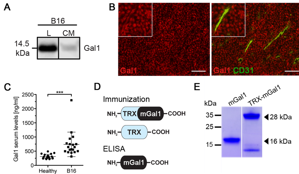
Fig. 1 Generation of a Gal1 vaccine for experimental melanoma. a Western blot for Gal1 in cell lysate (L) and conditioned media (CM; methanol-precipitated) from cultured B16 melanoma cells. b Immunostaining for Gal1 (red) and blood vessels (CD31, green; right panel) in tumors derived from B16 melanoma cells. Scale bar: 100 \mu m. c Gal1 measured in serum from healthy and tumor-bearing mice using a sandwich ELISA. Each dot represents an individual. The
