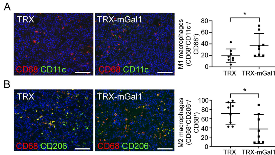
Fig. 5 Gal1 immunized mice have more M1 and less M2 macrophages compared to control immunized mice. a Representative immunostaining (CD68 and CD11c) and quantification of M1 macrophages in tumors from TRX (control) and TRX-mGal1 immunized mice ( p=0.0379 ). b Representative immunostaining (CD68 and CD206) and quantification of M2 macrophages in tumors from TRX (control) and TRX-mGal1 immunized mice ( p=0.0477 ). For
