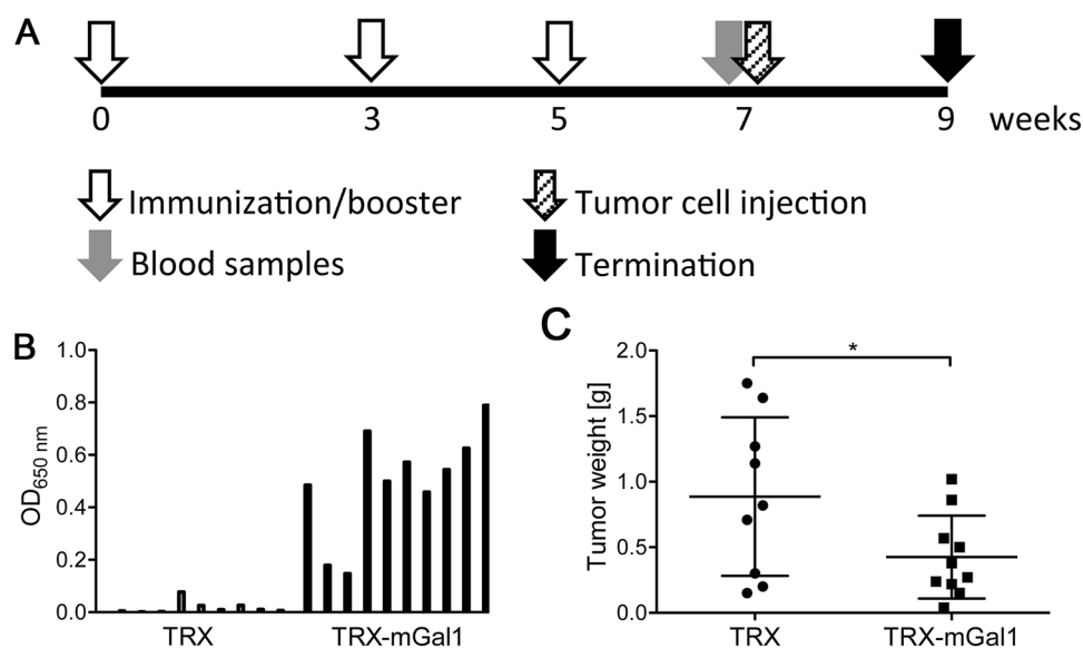
Fig. 2 Vaccination against Gal1 generates anti-Gal1 antibodies and suppresses tumor growth. a Immunization schedule for C57/BL6 mice with TRX (control) or TRX-mGal1 protein; time points for blood sampling, tumor challenge and termination are indicated. b Anti-Gal1 antibody levels measured by ELISA in serum from TRX and TRX-mGal1 vaccinated mice two weeks after the second booster
