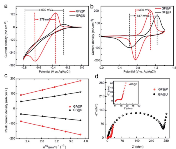
Fig. 4 (a) and (b) Cyclic voltammeteries of V^{3+}/V^{2+} and VO_2^{2+}/VO_2^+ redox using GF@U and GF@P electrodes at a scan rate of 10 \text{ mV s}^{-1} . (c) The relationship between GF@U and GF@P peak current density and square root of sweep speed. (d) Impedance diagram of GF@U and GF@P.
