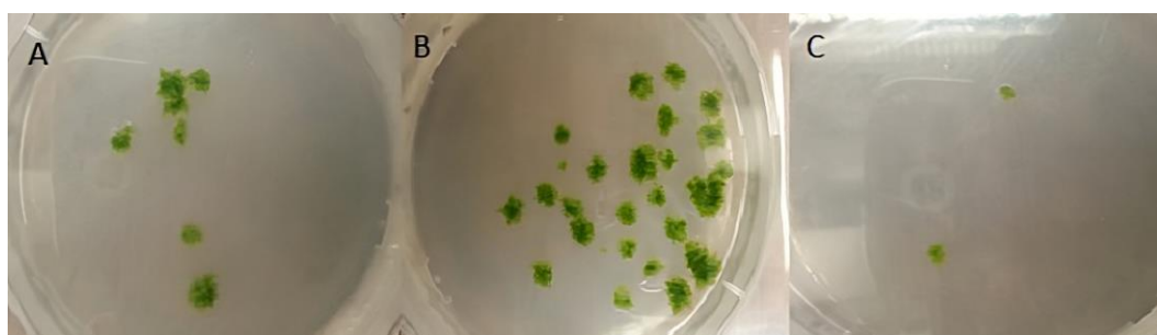
Figure 4. Stable P. patens transformants of the three transformation events after two rounds of selection. (A) transformants with ADS gene; (B) transformants with ADS and CYP71AV1-ADHI genes; (C) transformants with ADS , CYP71AV1-ADHI , and DBR2-ALDHI .
