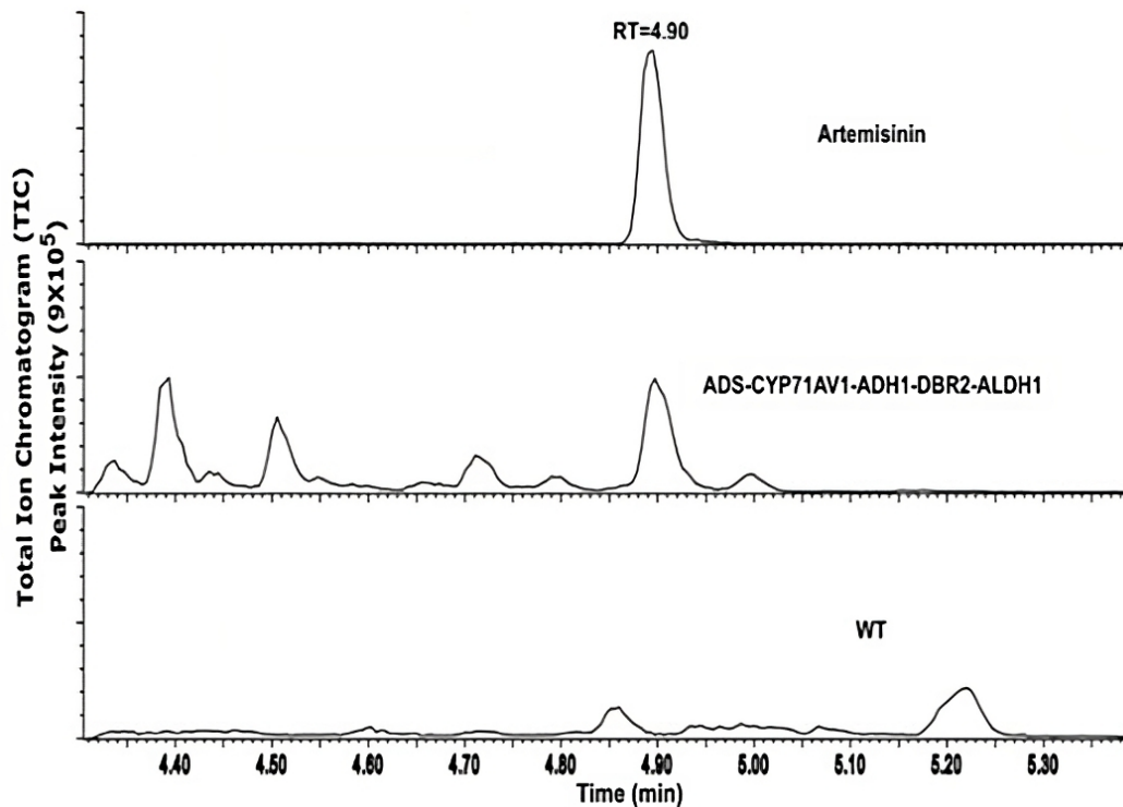
Figure 5. UPLC-MRM-MS analysis of transgenic Physcomitrium patens . Chromatogram of artemisinin standard (top), transgenic P. patens (middle), and wildtype P. patens (bottom). Figure taken from Khairul Ikram et al. (2017).
