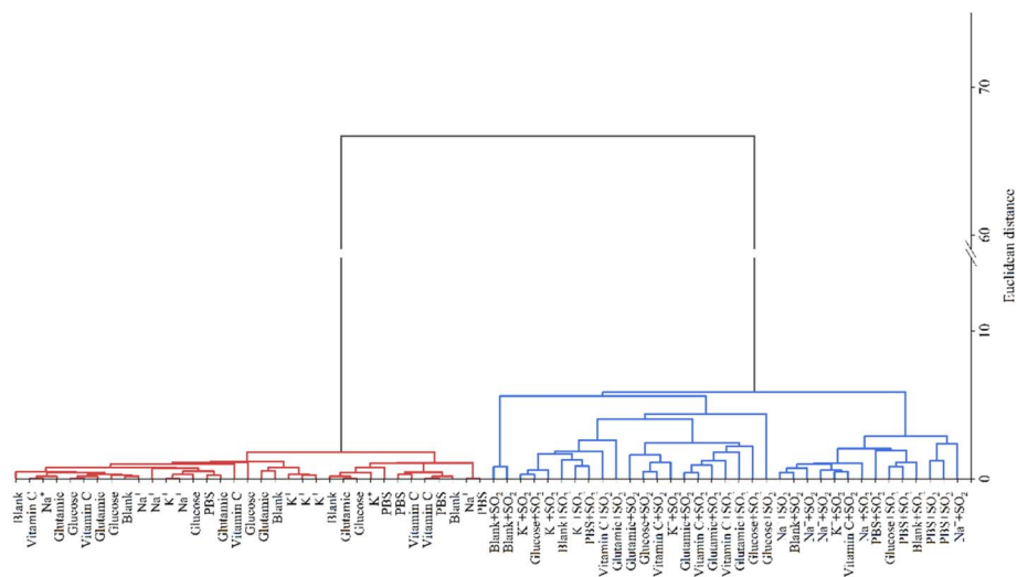
Fig. 4 Dendrogram of HCA of different interferences with and without sulfur dioxide. The final concentrations of interferences (e.g., blank, Na + , K + , PBS, vitamin C, glutamic acid, glucose) and sulfur dioxide were 100 \mu\text{g mL}^{-1} and 10 \mu\text{g mL}^{-1} , respectively.
