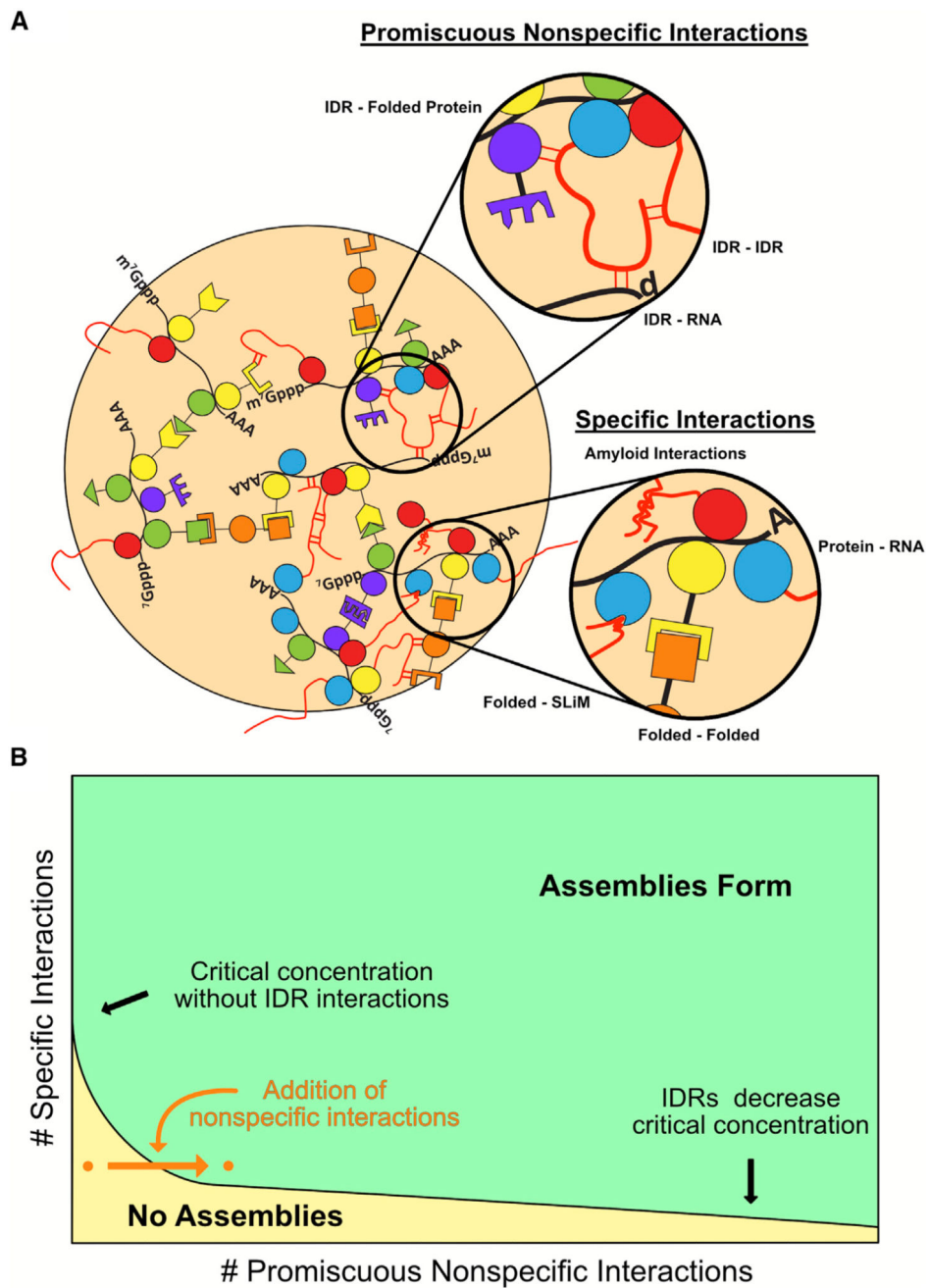
Figure 7. Model of RNP Granule Assembly and Contributions of IDRs A) RNP granules assembly by a wide variety of specific and nonspecific interactions. B) A theoretical phase diagram depicting how the addition of nonspecific, IDR-driven interactions could decrease the critical concentration of assembly for higher-order structures.
