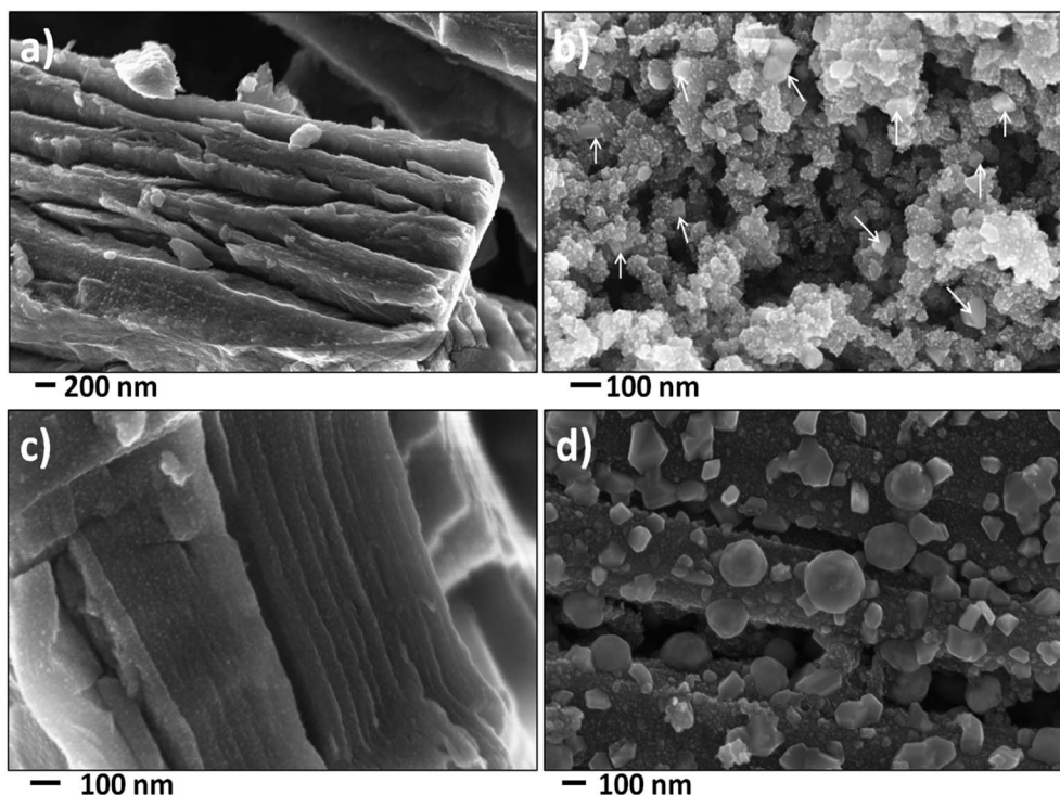
Fig. 3 High resolution SEM images of (a) PC–FeF 2 (b) CB–FeF 2 (c) G–FeF 2 and (d) CF–FeF 2 .
