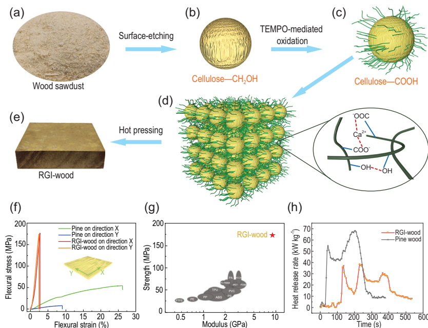
Figure 1. Schematic of the preparation and properties of regenerated isotropic wood. (a) Natural wood particles. (b) Surface-etched wood particle with cellulose microfibrils exposed from the surface. (c) Surface nanocrystallized wood particle (SNWP) with numerous cellulose nanofibers expanded from their surfaces. (d) Assembly of SNWP induced by Ca 2+ and hydrogen bonds. (e) The obtained RGI-wood by hot-pressing. (f) Flexural stress-strain curves of RGI-wood and natural wood in both directions. (g) Ashby plot: compared to other polymer-based materials, RGI-wood has outstanding mechanical performance. (h) The heat release rate curves of RGI-wood and natural pine wood given by cone calorimetry test showing that RGI-wood releases less heat during combustion. Adapted from Ref. [6].
