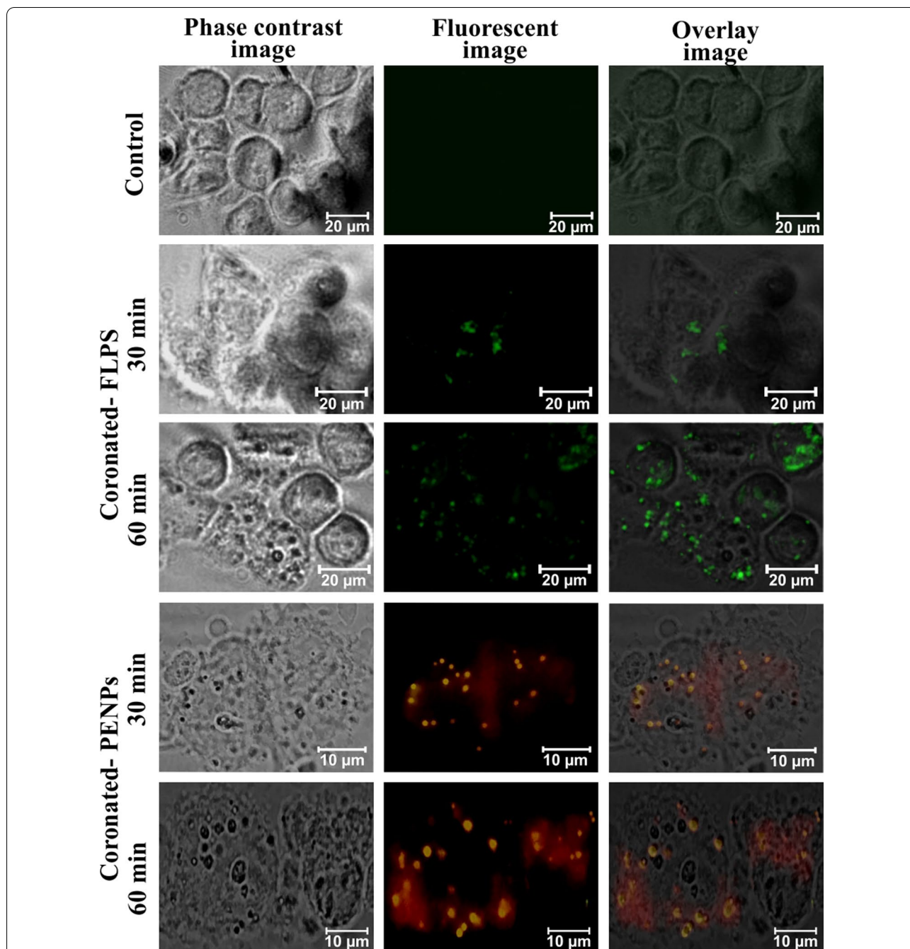
Fig. 7 Keratin-corona mediated rapid internalization of NPs in HaCaT cells. The phase-contrast, fluorescence, and superimposed images of HaCaT cells exposed to FLPS and Nile red stained PENPs particles. For the fluorescent imaging of coronated-FLPS and -PENPs, FITC fluorescent filter and I3 filter cube was used, respectively. Image arrangements from top to bottom: control, FLPS exposed for 30 min and 60 min, PENPs exposed for 30 and 60 min, respectively. The fluorescent-NPs without keratin-corona was used as a control
