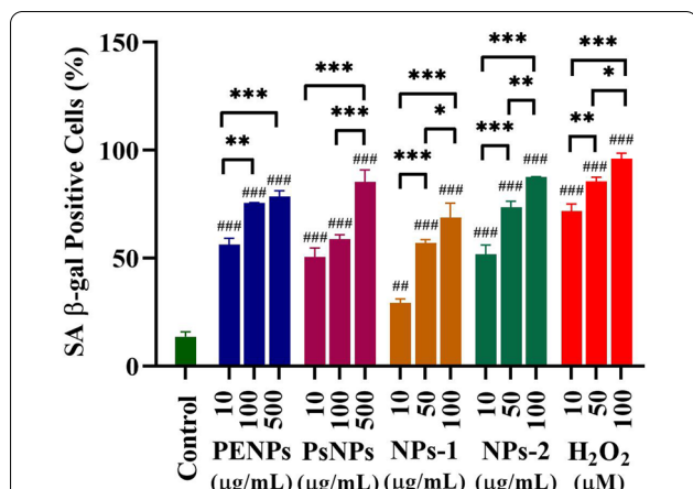
Fig. 11 Quantification of SA-β-gal positive cells that are treated with PENPs (10, 100 & 500 μg mL -1 ), PSNPs (10, 100 & 500 μg mL -1 ), NPs-1 (10, 50 & 100 μg mL -1 ), and NPs-2 (10, 50 & 100 μg mL -1 ) and H 2 O 2 (10, 50 & 100 μM) for 48 h and then incubated with fresh, NPs-free medium. Micrographs were obtained with phase-contrast microscopy. Totally 250 cells scored from five images were expressed as the percentage (mean ± SEM) of positive cells. * p < 0.05, ** p < 0.01, *** p < 0.001 significantly different from the same NPs concentration. # p < 0.05, ## p < 0.01, ### p < 0.001 significantly different from the control
