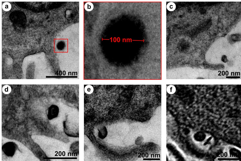
Fig. 8 Mechanism of NPs internalization in HaCaT cells. a Binding of coronated NPs on keratinocytes surface, b magnified view of NPs on the cells surface, c, d pinocytotic cups/large membrane ruffles formation, e membrane ruffles folding back on the cell surface along with the coronated NPs and f membrane surrounded intracellular compartment
