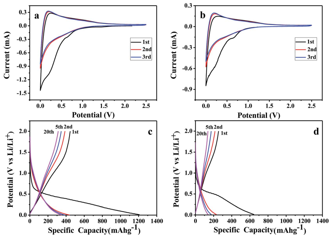
Fig. 5 Cyclic voltammograms of (a) N-GP and (b) GP electrodes at a scan rate of 0.2 \text{ mV s}^{-1} between 0.01 \text{ V} and 2.5 \text{ V} vs. \text{Li}/\text{Li}^+ ; and galvanostatic charge/discharge profiles of (c) N-GP and (d) GP electrodes at a specific current of 100 \text{ mA g}^{-1} between 0.01 \text{ V} and 2.0 \text{ V} vs. \text{Li}/\text{Li}^+ .
