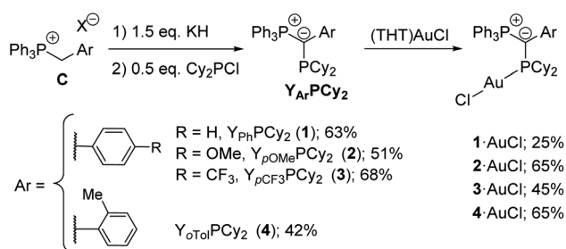
Scheme 1 Preparation of the YPhos ligands 1–4 .
