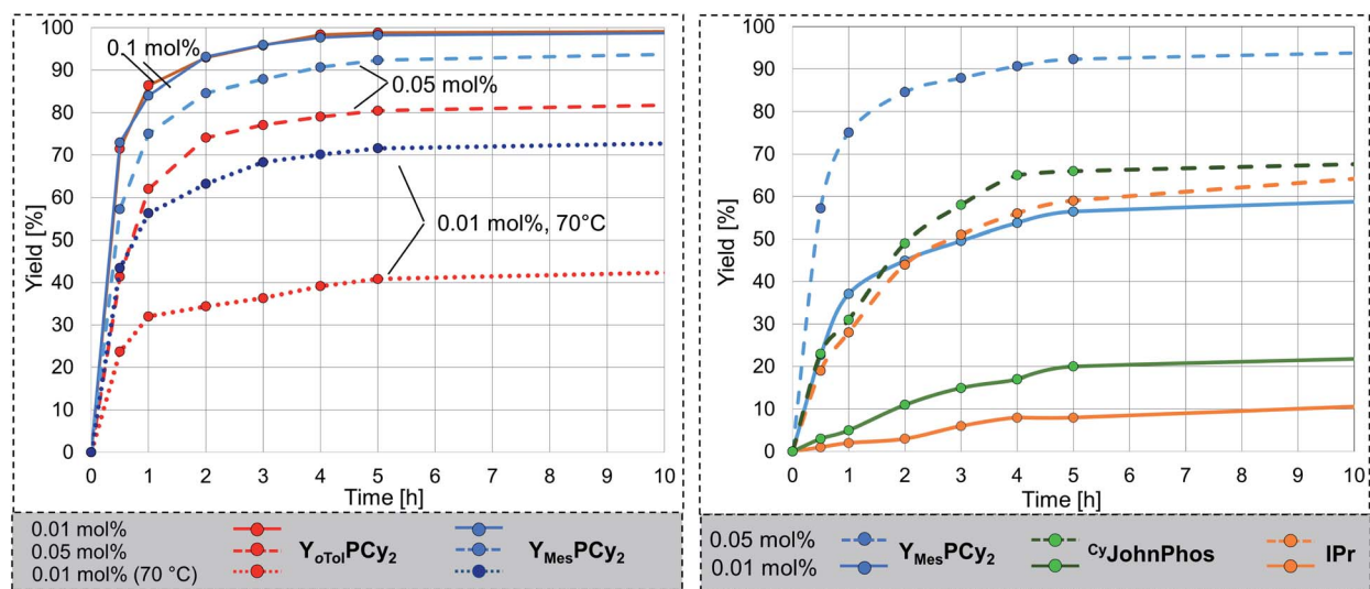
Fig. 6 (Left) Comparison of the catalytic activity of the gold complexes with 4 and 5 at different catalyst loadings; (Right) comparison of the activity of the AuCl complexes of 5 , IPr and \text{CyJohnPhos} at 0.05 and 0.01 mol% catalyst loading. Reaction conditions: aniline (1 eq.), phenylacetylene (1 eq.), gold complex : \text{NaBAR}^{\text{F}} = 1 : 1, 50^\circ\text{C} (if not stated otherwise). Conversion was determined by NMR spectroscopy.
