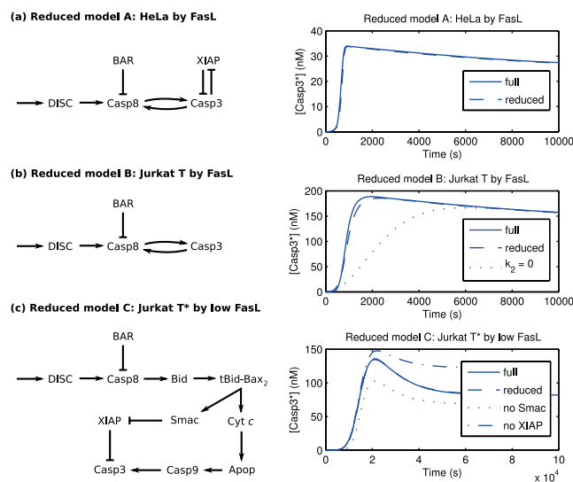
Figure 5 Reduced models under induction by FasL. Reduced models of apoptosis under induction by FasL (receptor-mediated apoptosis; [FasL]_0 = 2 \text{ nM} unless noted), with time course validations. In (a) and (c), the time courses of the full and reduced models essentially overlap. (a) HeLa cell induced by FasL. (b) Jurkat T cell induced by FasL. (c) Jurkat T* cell induced by low FasL ( [FasL]_0 = 0.01 \text{ nM} ).
