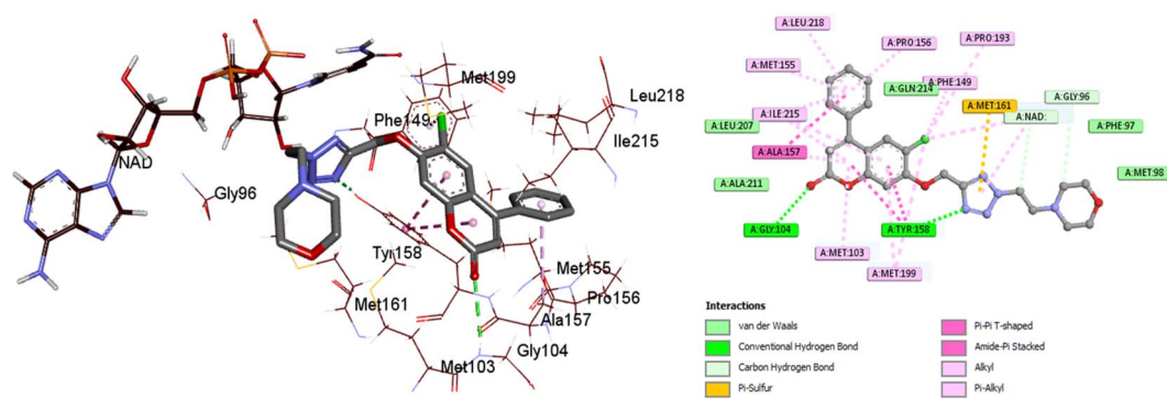
Fig. 8 2D and 3D interaction maps between InhA residues and ligand 4c.
