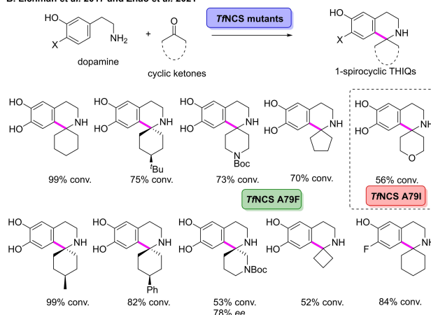
Scheme 16. (A) Pictet-Spengler reaction between dopamine and a number of substituted methyl ketones catalysed by norcochlorine synthase mutants. (B) Pictet-Spengler reaction between dopamine with cyclic ketones catalysed by norcochlorine synthase mutants.
