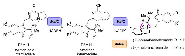
Scheme 14. Biocatalytic synthesis of (+)-malbrancheamide involving the bifunctional NADPH-dependent reductase/Diels-Alderase MalC .
