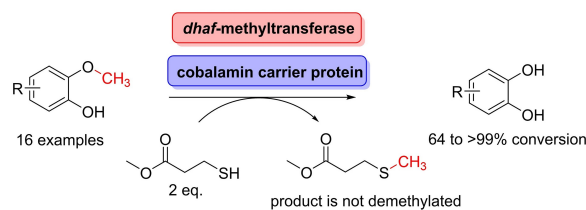
Scheme 33. Enzymatic demethylation employing cobalamin-dependent methyltransferases using thiols as methyl acceptors.
