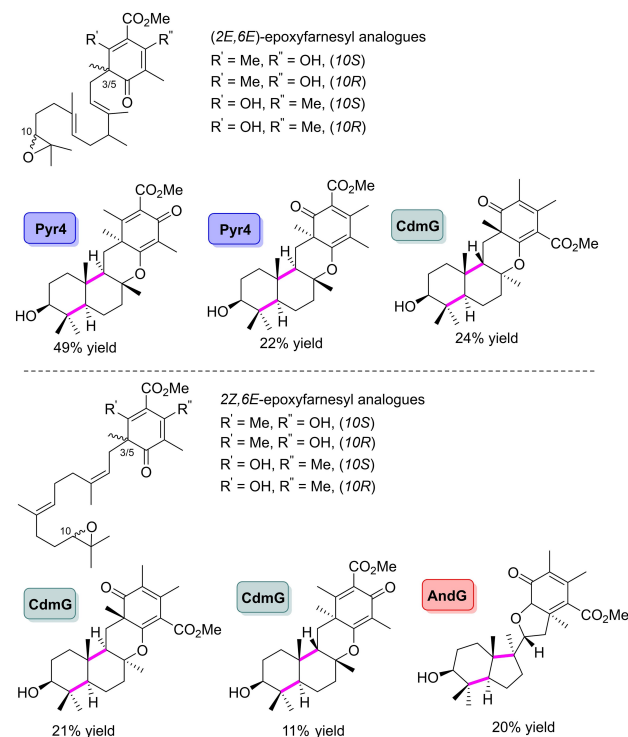
Scheme 10. Enzymatic polycyclisation of synthetic epoxyfarnesyl analogues catalysed by a number of meroterpenoid cyclases.
