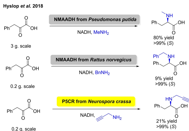
Scheme 30. N -Methyl amino acid dehydrogenases (NMAADHs/DpkAs), ketimine reductases (KIREDs), and pyrroline-5-carboxylate reductases (P5CRs) for the synthesis of N -alkylated amino acids.
