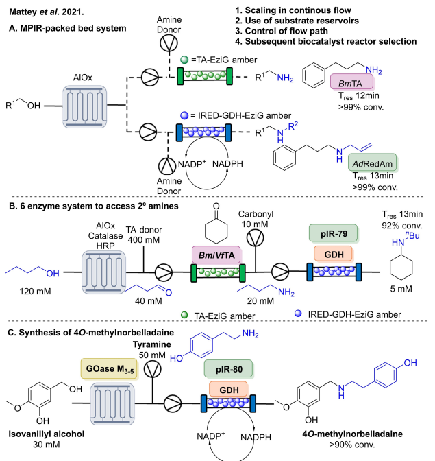
Scheme 24. IREDs in flow. (A) An overview of the MPIR-packed bed system with the AIOx (alcohol oxidase) in cascade with the either a transaminase (TA) or IRED. (B) A 6-enzyme compartmentalised system to access secondary amines. (C) Combining GOase M 3-5 with pIR-80 to access 4O-methylnorbelladaine from isovanillyl alcohol and tyramine.
