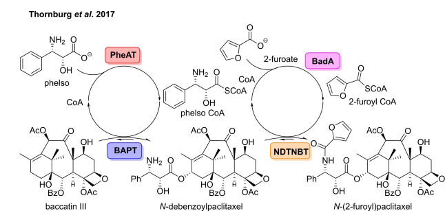
Scheme 3. Four enzyme cascade for the preparation of paclitaxel analogues starting from commercially available baccatin III.
