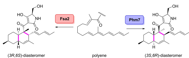
Scheme 12. Diastereoselective Diels-Alderases in the synthesis of decalin scaffolds.
