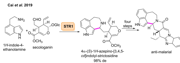
Scheme 19. Enzyme catalysed Pictet-Spengler reaction of non-natural 1 H -indole-4-ethanamine towards azepino-indole scaffolds.
