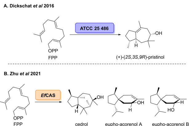
Scheme 7. Novel STCs to access 5–8 bicyclic sesquiterpene alcohols.
