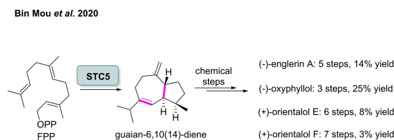
Scheme 8. Highly stereoselective enzymatic synthesis of guaian-6,10(14)-diene precursor prior to chemical transformation to biologically active epoxy-guaiane sesquiterpenes.
