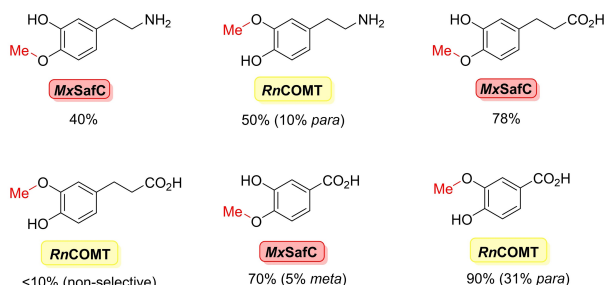
Scheme 31. Substrate scope, conversions and regioselectivity displayed by the catechol O -methyltransferases from Myxococcus xanthus ( MxSafC ) and Rattus norvegicus ( RnCOMT ).
