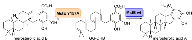
Scheme 9. A novel terpene cyclase catalysed polycyclisation of GG-DHB to merosterolic acid A in the biosynthesis of cytotoxin merosterol A.
