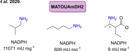
Scheme 29. The scope and applications of natural and metagenomic AmDHs. (A) First example of wild-type AmDHs, AmDH4 in the reductive amination of 4-oxopentanoic acid. (B) Exploration of wild-type genomic AmDHs with the enzyme studied listed in the table with example of the scope and specific activity mU mg -1 given below each product. (C) Exploration of metagenomics resources for the discovery of new AmDHs.
