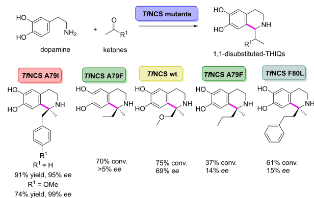
Scheme 17. Pictet-Spengler reaction between dopamine and a panel of substituted benzaldehydes catalysed by wild type norcochlorine synthase (NCS).
