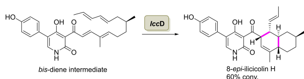
Scheme 13. (A) A novel Diels-Alderase, PvhB , catalyses the endo -selective Diels-Alder reaction of the carboxylate intermediate in the biosynthesis of varicidin A. (B) Enzymatic IED Diels-Alder reaction of bis -diene to furnish 8- epi -ilicicolin H catalysed by a novel Diels-Alderase, IccD .
