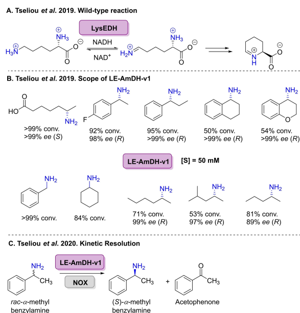
Scheme 28. The scope and applications of the engineered \epsilon -deaminating L-lysine dehydrogenase from Geobacillus stearothermophilus . (A) The wild-type reaction is outlined. (B) Examples of the scope and selectivity of the LE-AmDH-v1 variant at 50 mM substrate concentration. (C) Application LE-AmDH-v1 combined with a NOX to allow of the kinetic resolution of primary amines, where the scope was similar to that shown in B.
