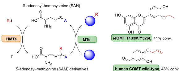
Scheme 32. Novel strategies for general enzymatic O -alkylation involving methyltransferases using (A) stoichiometric naturally occurring SAM derivatives and (B) in combination with halide methyltransferases to generate artificial SAM derivatives.
