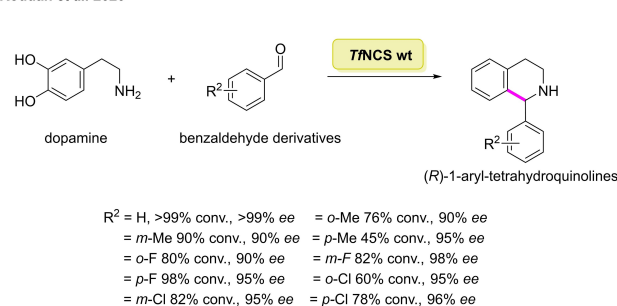
Scheme 17. Pictet-Spengler reaction between dopamine and a panel of substituted benzaldehydes catalysed by wild type norcochlorine synthase (NCS).
