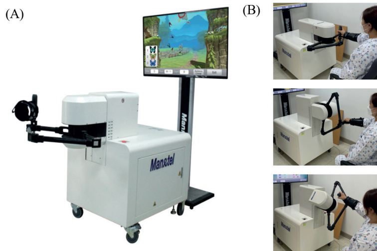
Fig. 1. (A) Camillo® set up (3DBT-61, Man&Tel Co. Ltd, Gumi, Republic of Korea), an end effector type of electromechanically-assisted upper limb training device. (B) Three positioning modes of training; horizontal, vertical and inclined plane
