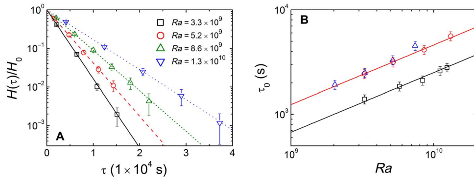
Fig. 4. Statistical properties of the time interval \tau between adjacent eruption events. (A) Normalized histogram H(\tau)/H_0 as a function of \tau for the 10% glycerin solution at four different values of Ra . The error bars indicate the SD of the measurements. The color-coded lines show the exponential fits, H(\tau)/H_0 \approx \exp(-\tau/\tau_0) , to the data points with \tau_0 = 2430 s (black solid line), 3150 s (red dashed line), 4140 s (green short dashed line), and 5600 s (blue dotted line). (B) Obtained mean time interval \tau_0 between adjacent eruption events as a function of Ra for three different fluids: water (blue triangles), 10% glycerin solution (red circles), and 20% glycerin solution (black squares). The error bars show the experimental uncertainty of the measurements. The solid lines (color coded) are the power-law fits, \tau_0 = aRa^\beta , to the data points, with a = 0.0092 and \beta = 0.57 \pm 0.1 for the red circles and a = 0.005 and \beta = 0.57 \pm 0.1 for the black squares.
