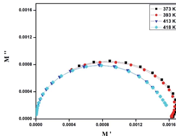
Fig. 13 Complex modulus spectrum of [\text{TPA}]_2\text{CoBr}_4 at selected temperatures.
