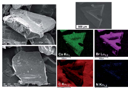
Fig. 1 SEM images of large [(\text{C}_3\text{H}_7)_4\text{N}]_2\text{CoBr}_4 crystals grown by slow evaporation method at room temperature and EDS elemental Co, Br, C and N maps collected on two V-shape twinned crystals.
