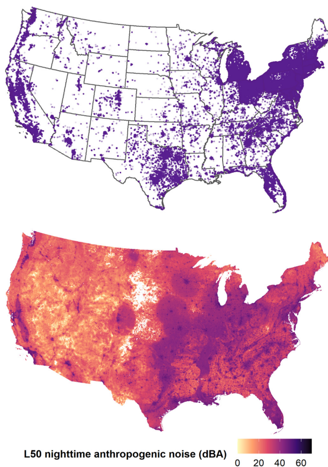
Figure 1. Location of Nurses' Health Study addresses ( n participants = 114,116) from 1988–2018 (above) and map of anthropogenic nighttime L_{50} sound (dBA) in 2000–2014 (below). Note: L_{50} , noise level exceeded 50% of the time.
