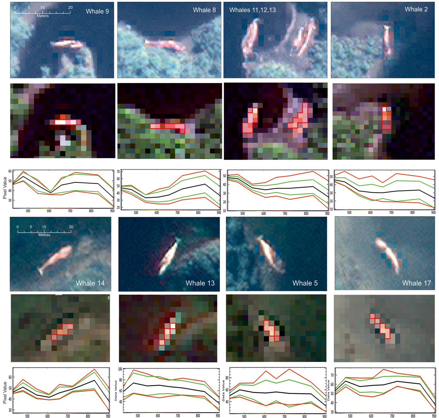
Fig 4. Image chips and spectral profiles from ten whales. At the top are whales from Image 1 and the bottom are from Image 2. The upper row displays detailed pan-sharpened images (spatial resolution 0.5 m) shown using visible bands of the satellite imagery. The second row is the multispectral band (2 m resolution pixels) used in the spectral analysis with the area of pixels chosen for each profile highlighted in red. The third row are the spectral profiles for each image showing Top-Of-Atmosphere radiance in the Y axis and wavelength in nanometers in the X axis. Imagery from DigitalGlobe Products. WorldView2 © 2019 DigitalGlobe, Inc., a Maxar company.
