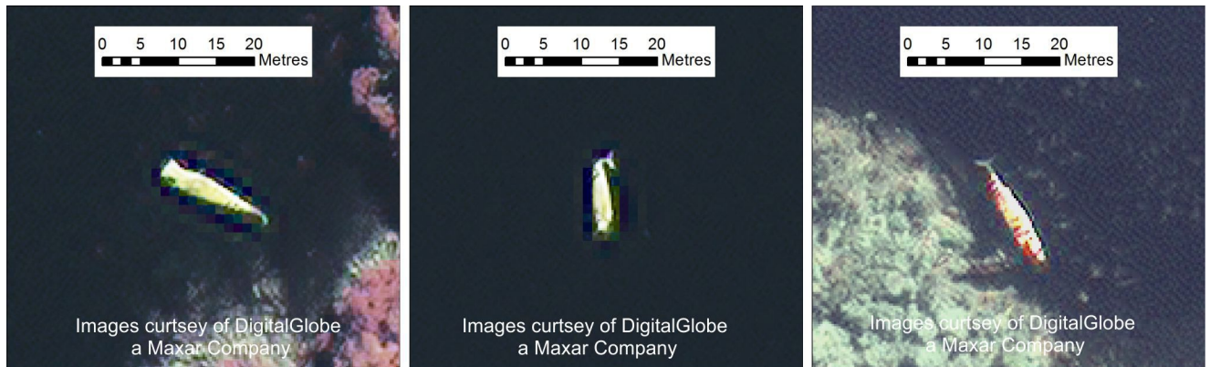
Fig 5. Examples of stranded whales in WorldView3 imagery from the Gulf of Penas in March 2017, showing the improved shape discrimination using this higher resolution data. The locations of these whales are shown as blue triangles in Fig 1. Imagery from DigitalGlobe Products. WorldView3 © 2019 DigitalGlobe, Inc., a Maxar company.
