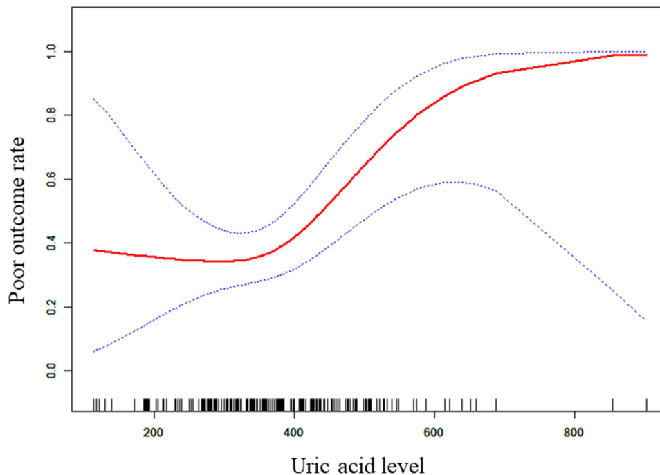
Figure 2 The threshold effect of uric acid levels on short-time prognosis outcome of ICH patients.
