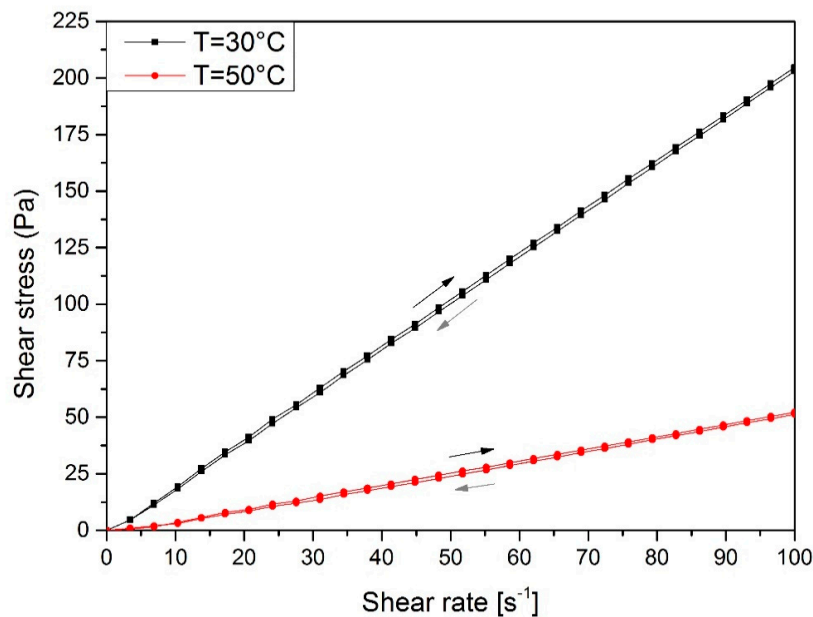
Figure 4. The flow curves of obtained polyol at different temperatures.
