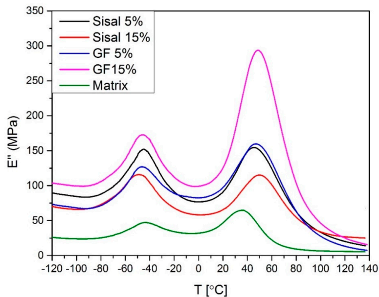
Figure 10. Loss modulus values of obtained hybrids.
