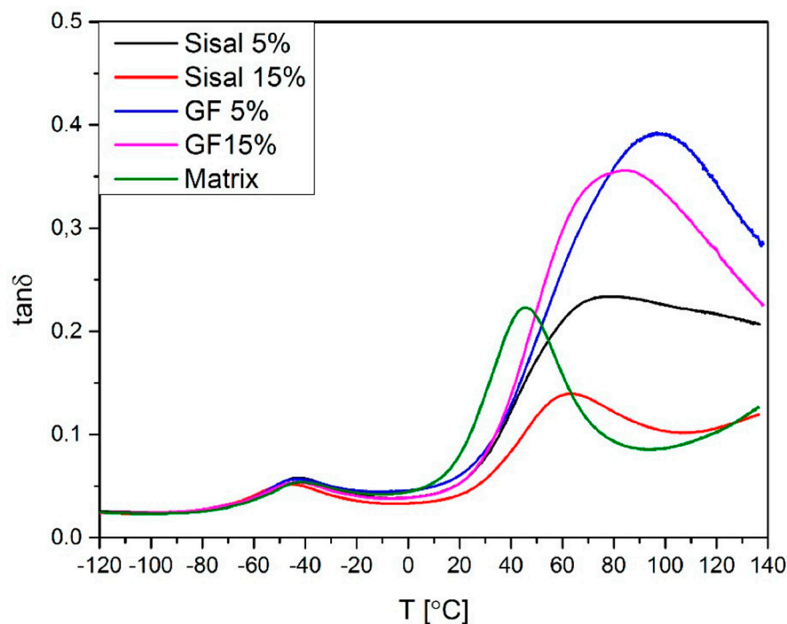
Figure 12. Loss factor ( \text{Tan}\delta ) values of obtained composites.
