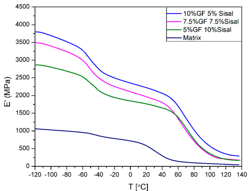
Figure 9. Storage modulus values of obtained hybrids.
