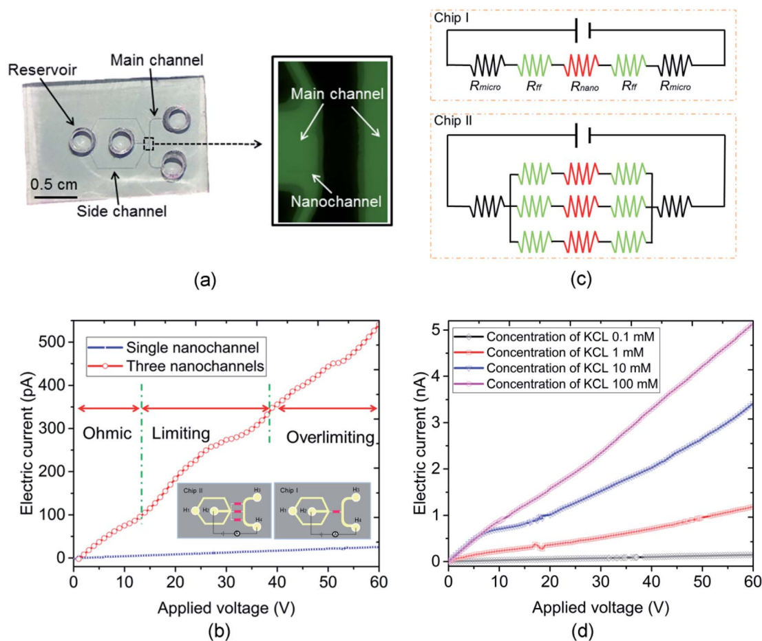
Fig. 2 (a) Schematic diagram of nanofluidic chip, (b) electric current measurement results of chips I and II, (c) an equivalent electrical circuit of chips I and II that comprised of resistors, and (d) electric current measurement results for concentration of KCl from 0.1 to 100 mM.
