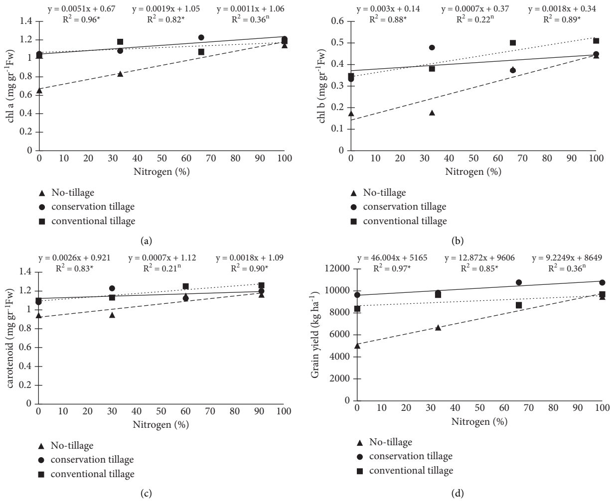
FIGURE 2: The trend of nitrogen fertilizer changes on chlorophyll a (a), chlorophyll b (b), carotenoids (c), and grain yield (d) of corn under tillage treatments.
