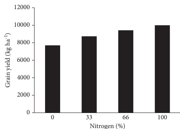
FIGURE 4: Effect of nitrogen fertilizer on grain yield of corn.
