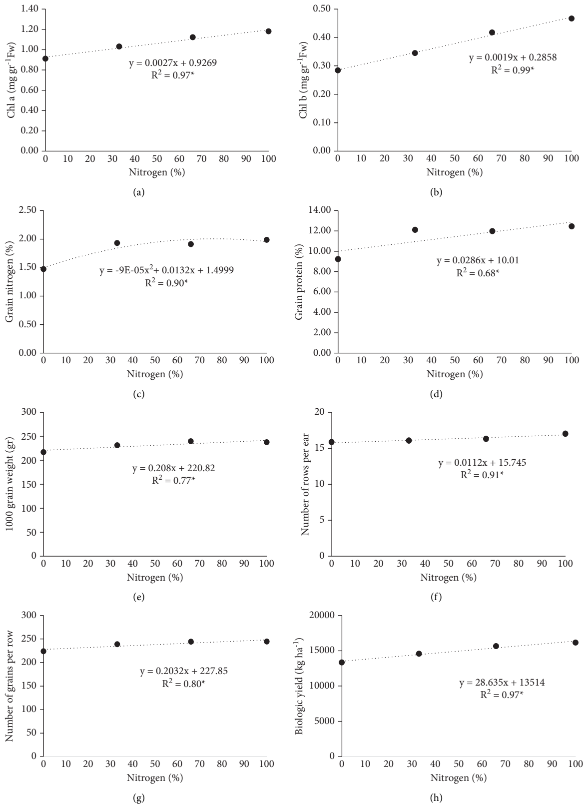
FIGURE 1: The trend of changes in nitrogen fertilizer levels on chlorophyll a (a), chlorophyll b (b), grain nitrogen (c), grain protein (d), 1000-grain weight (e), number of rows per ear (f), number of grains per row (g), and biological yield (h).
