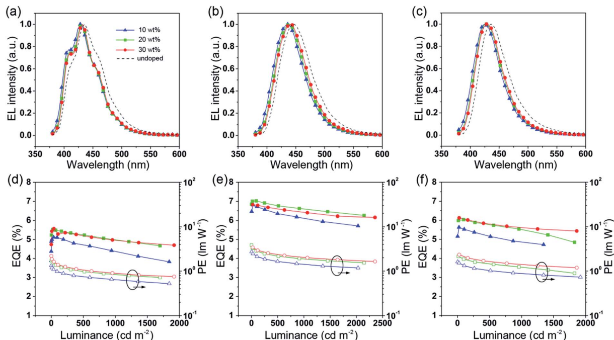
Fig. 6 EL spectra of the CBP-doped devices based on (a) TPICz, (b) TPINCz and (c) TPIBNCz. The EQE–luminance curves for the CBP-doped devices based on (d) TPICz, (e) TPINCz and (f) TPIBNCz.
