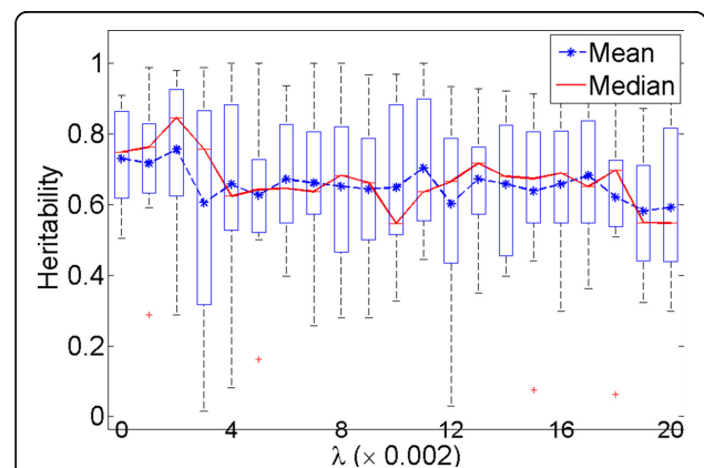
Figure 5 Case study on cocaine dataset: the testing h^2 of the composite traits derived in three-fold cross validation with varying \lambda .
