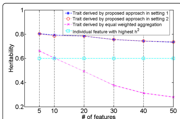
Figure 3 Simulation study: comparison of h^2 of commonly used traits with that of the quantitative traits derived by the proposed approach with chosen \lambda 's. Results from both settings (setting 1 - without covariates, setting 2 - with covariates) are shown. For h^2 of individual features in each dataset, we show the highest. Because in our simulation the feature that has the highest h^2 estimate is shared across all the datasets with varying number of features, the corresponding h^2 curve is a straight line. Since covariates do not affect the h^2 estimate when their effect is properly corrected for during the estimation, we do not differentiate the two settings and show one curve for traits derived by equal weighted aggregation of individual features in the data and one for individual feature that has the highest h^2 estimate.
