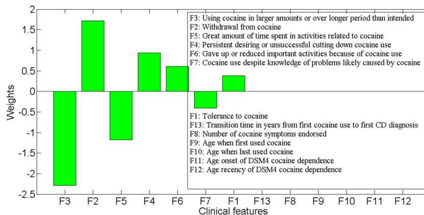
Figure 6 Case study on cocaine dataset: the weights of variables in the linear combination learned by the proposed method with \lambda = 4 and the entire sample set.
