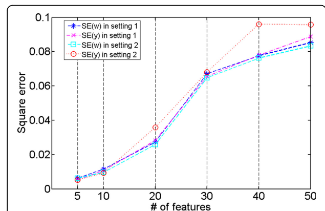
Figure 4 Simulation study: the square error of feature weights (w) in models derived by the proposed approach with chosen \lambda 's: SE(w) and that of resulted quantitative traits (y): SE(y), comparing to the optimal (implanted) model coefficients ( \hat{w} ) and traits ( \hat{y} ). SE(w) is calculated as \|\mathbf{w} - \hat{\mathbf{w}}\|_2^2 ; and SE(y) is calculated as \|\mathbf{y} - \hat{\mathbf{y}}\|_2^2/n , where n is the total number of subjects in 2 2 the data. Results from both settings (setting 1 - without covariates, setting 2 - with covariates) are shown.
