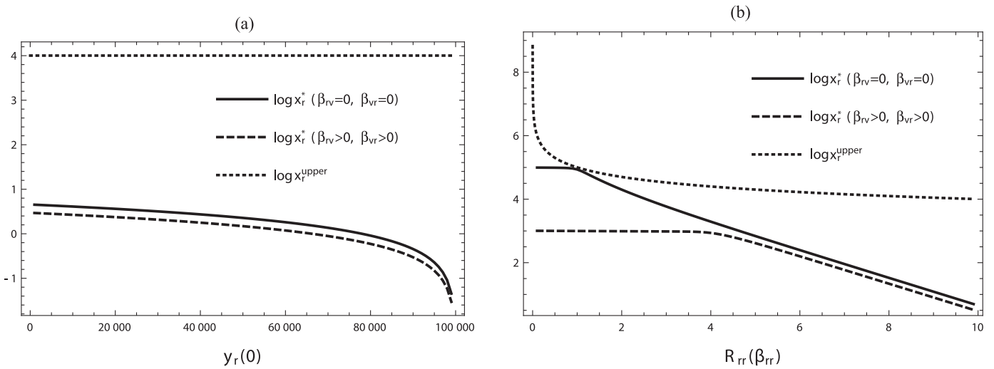
Fig. 3. The dependence of the final size of susceptible resident population x_r^* on the initial size of infective resident population y_r(0) and on \beta_{rr} . (a) \beta_{rv} = 2.0 \times 10^{-5}, \mathcal{R}_{rr} = 10.0, (x_r(0), y_r(0), y_v(0)) = (N_r - y_{r0}, y_{r0}, 0.0) ; (b) (x_r(0), y_r(0), y_v(0)) = (99990.0, 10.0, 0.0) . The horizontal axis in (b) shows the value of \mathcal{R}_{rr} which is a function of \beta_{rr} as given by (4). Commonly, N_r = 100000.0, N_v = 100.0, \rho = 0.2, M = 0.5, \beta_{vr} = 1.6 \times 10^{-4}, \beta_{rv} = 1.0 \times 10^{-5}, \beta_{vv} = 4.0 \times 10^{-5}, \mathcal{R}_{vv} = 0.8, \mathcal{R}_{vr} = 0.08, \mathcal{R}_{rv} = 200.0 .
