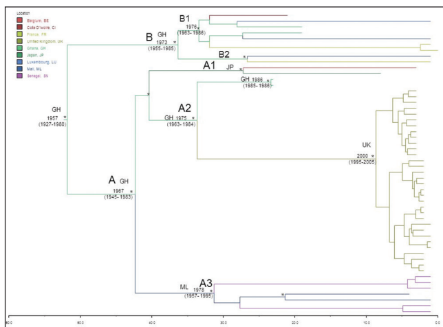
Figure 1: Bayesian phylogeographic tree of HIV-2 Group B pol gene sequences. The branches are colored on the basis of the most probable state location of the descendent nodes. States are reported on the left corner of the figure. The scale at the bottom of the tree represents time in years. Years are reported for the main nodes.
