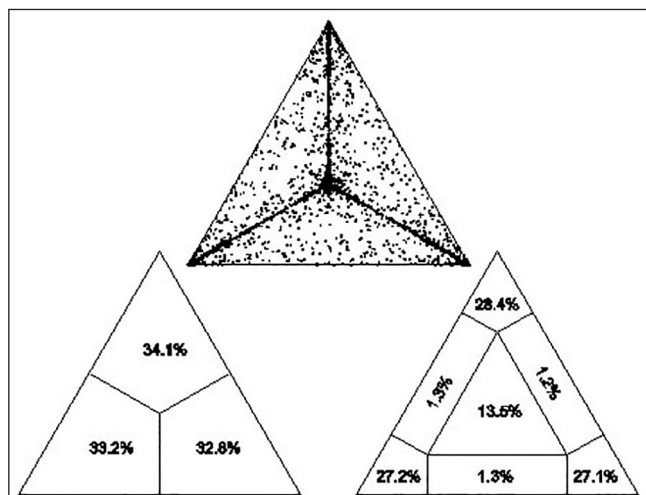
Supplementary Figure 1: Likelihood-mapping of HIV-2 Group B pol gene. The dots inside the triangles represent the likelihood of the possible unrooted topologies for each quartet. Numbers indicate the percentage of dots in the center of the triangle corresponding to phylogenetic noise (star-like trees).
