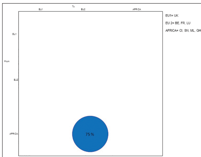
Figure 3: Maximum parsimony migration patterns of the HIV-2 Group B pol gene to and from different areas. The bubblegram shows the frequency of gene flow (migrations) to and from different areas. The surface of each circle is proportional to the percentage of observed migrations given within the circle. Migrations were inferred with a modified version of the Slatkin and Maddison algorithm.
