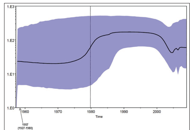
Figure 2: Bayesian skyline plot of the HIV-2 Group B pol gene. The effective number of infections is reported on the Y-axis. Time is reported on the X-axis. The colored area corresponds to the credibility interval based on 95% highest posterior density interval.
