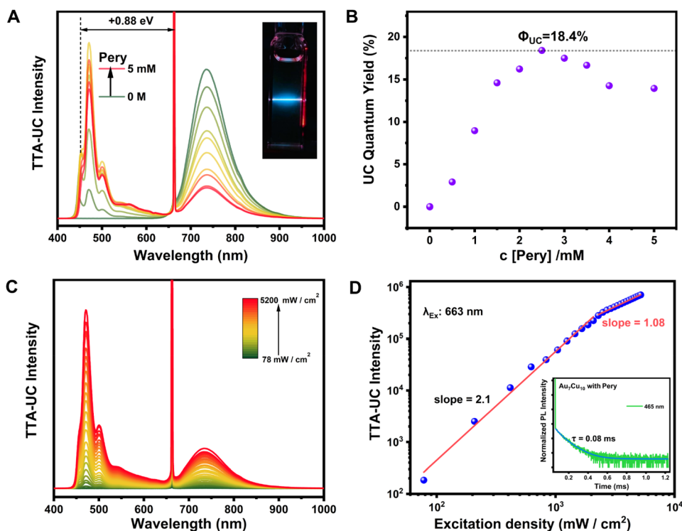
Fig. 4 (A) PL spectra of \text{Au}_7\text{Cu}_{10} and Pery at various concentrations with excitation at 663 nm, where the inset shows the photograph of the TTA-UC emission process. (B) Relationship of the TTA-UC quantum yield with the Pery concentration. Note that the theoretical maximum of \Phi_{\text{UC}} is defined as 100%. 73 (C) Dependence of the TTA-UC fluorescence intensity on the excitation power density. (D) Double logarithmic plot of the integrated TTA-UC fluorescence intensity with the excitation power density, where the inset shows the lifetime measurement of delayed fluorescence of Pery.
