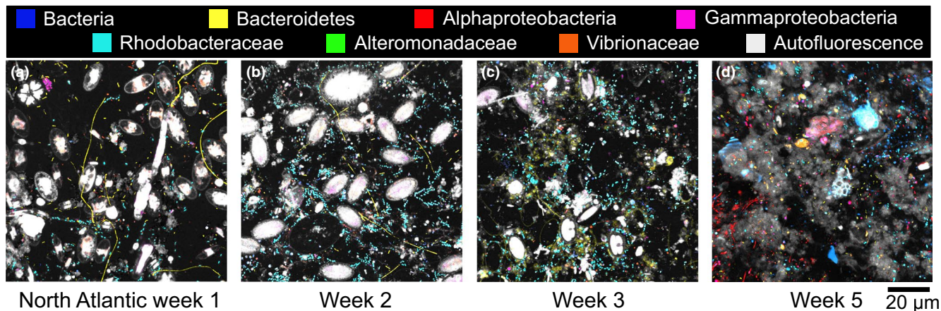
FIGURE 3 Succession of the biofilm community on polyethylene (PE) after 1–5 weeks in the surface (~1 m) of the North Atlantic Ocean (Vineyard Sound), Woods Hole, MA, USA. The black background is the surface of the plastic pieces. Elliptical white structures are diatom (phytoplankton) cells attached to the PE surface, and are visible due to their autofluorescent pigments such as chlorophyll a . Various coloured smaller cells are bacteria hybridized with phylogenetic probes targeting different levels of taxonomic resolution. Greyish and coloured material in the week 5 sample are unidentified organic material (perhaps biofilm EPS) with captured autofluorescent pigments making these structures visible
