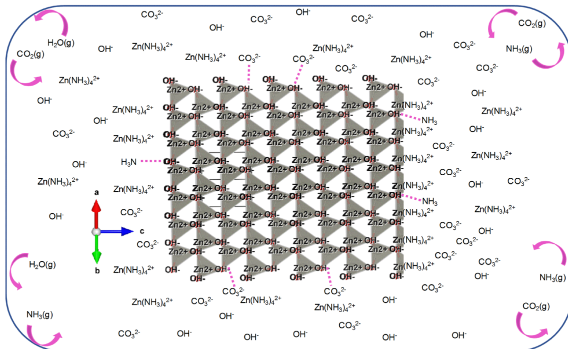
Figure 3. Schematic of a representative PNC, and dynamism of the closed system. 3D hcp -like aggregations of Zn 2+ and OH - ions (without bonding) constitute the PNCs here. Though not drawn for clarity purpose, the Zn 2+ ions in these PNCs are stabilized by ammonia complexation—as Zn(NH 3 ) 4 2+ . The extent of PNCs is defined by the temporal solution properties, which keep fluctuating throughout the process. PNCs initially co-exist with non-dense regions. Representative ions/species in the non-dense region is shown around the PNC. The dotted lines represent possible hydrogen bonds between species (This is only qualitative representation, not quantitative). Nucleation starts within the PNCs on expulsion of gaseous molecules, especially ammonia complexed with Zn 2+ ions that stabilizes these PNCs, and carbonates. The growth follows by the aggregate addition of crystallites formed from these PNCs. Dynamism of gaseous molecules is schematically represented.
