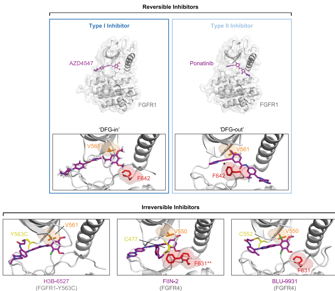
Figure 5. Binding modes of FGFR inhibitors.
