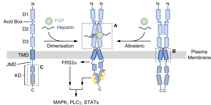
Figure 1. Stimulation of FGFRs.
