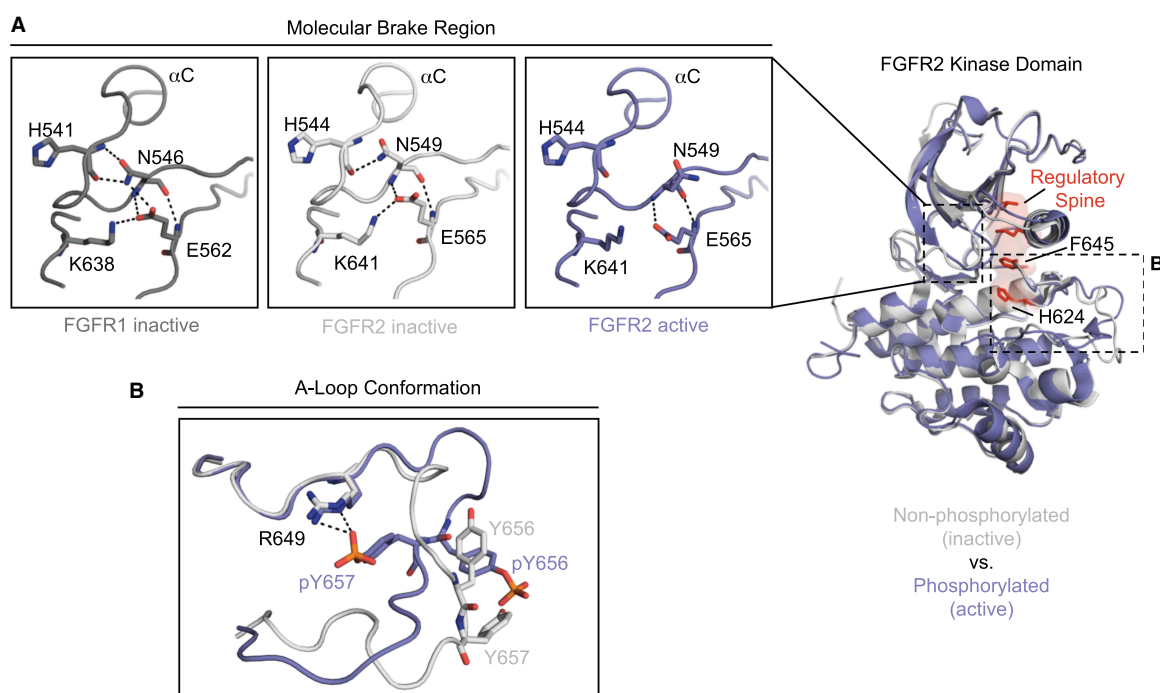
Figure 3. Comparison of active and inactive FGFR kinase domain states.
