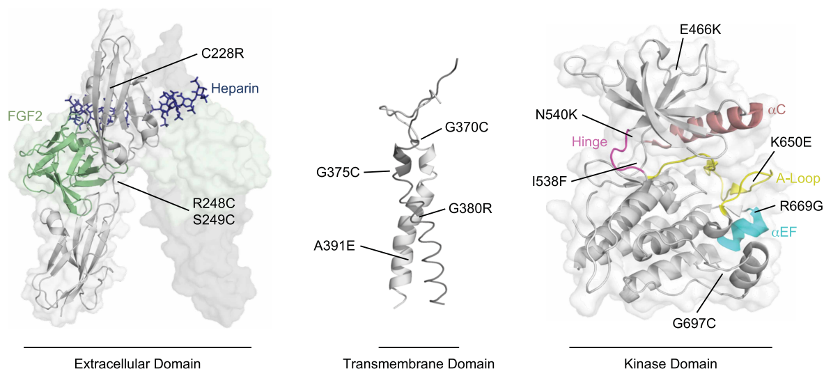
Figure 4. Point mutations of FGFR3.
