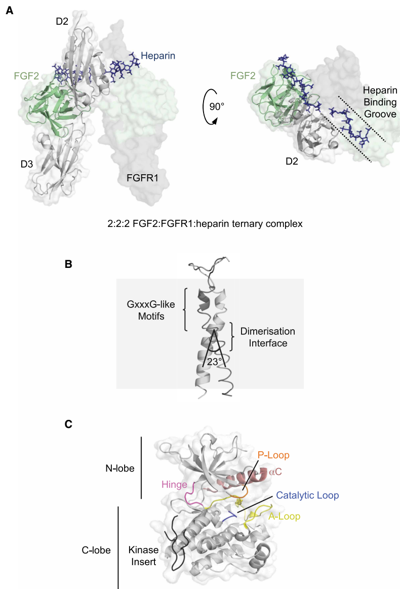
Figure 2. Structures of FGFR extracellular, transmembrane, and kinase domains.
