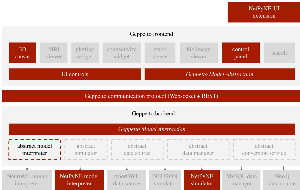
Figure 6. Geppetto NetPyNE-UI configuration. Graphical representation of the components of Geppetto that are used on the NetPyNE-UI application (red). The ones not used are coloured in grey.
