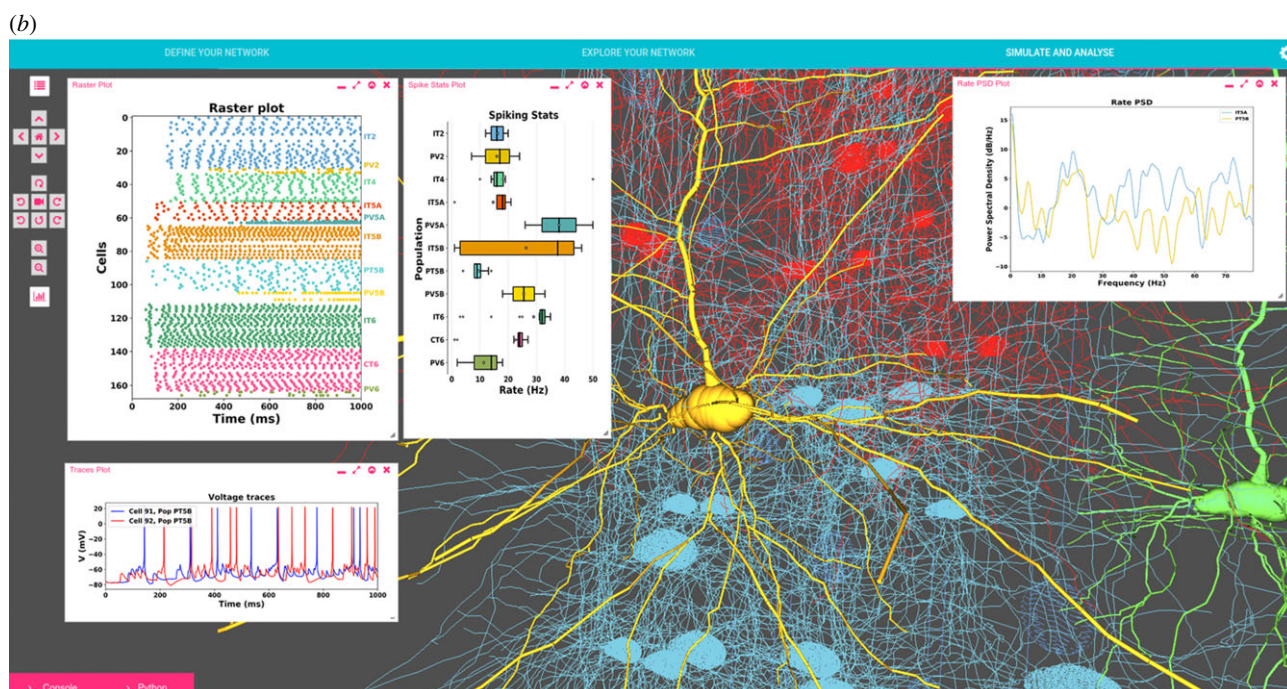
Figure 7. (a) Screenshot of NEURON-UI while in edit mode, a simplified cell builder (bottom left) lets the user edit any selected section (in yellow) while the Run control panel (right) is used to control the simulation. (b) NetPyNE-UI showing the result of a simulation of a large-scale M1 microcircuit model with widgets showing a raster plot (top left), individual cell membrane potentials (bottom left), population spiking statistics (middle) and the power spectral densities for two populations (right).
