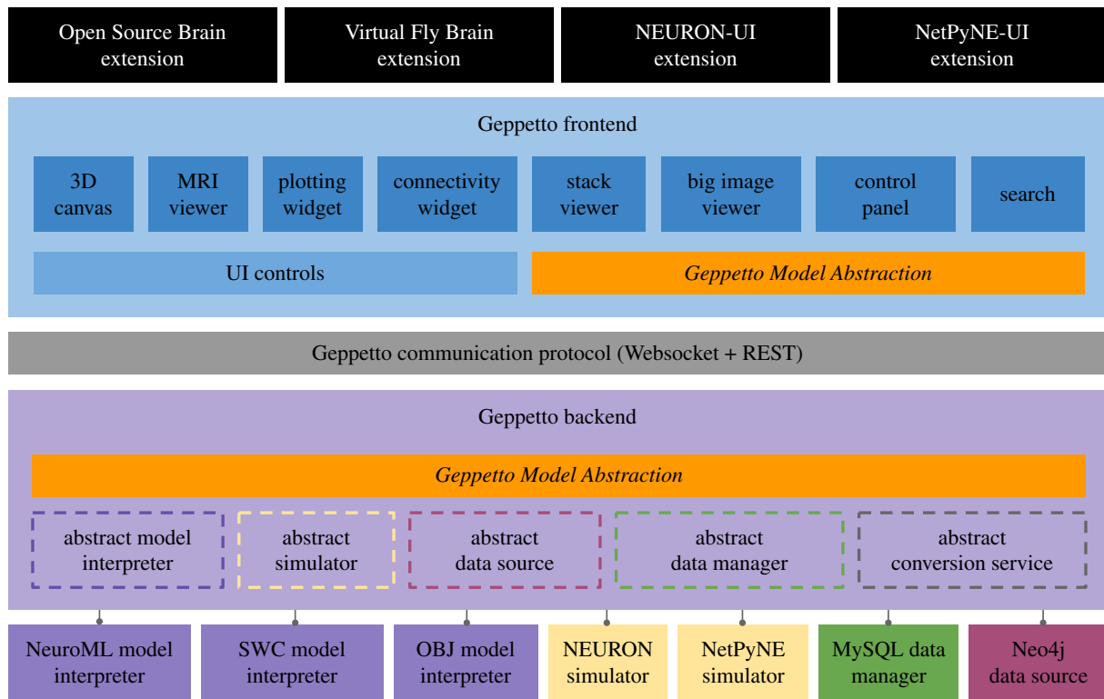
Figure 1. Geppetto architecture. Graphical representation of the components of Geppetto illustrating how the Geppetto Model Abstraction (orange blocks) allows backend model and data sources to be accessed by users through browser-based frontend components. Black blocks in the figure are Geppetto Extensions, used by applications built on top of the Geppetto platform. The Geppetto frontend (shades of blue) is shown containing a diverse set of visualization components. Communication between the frontend and backend happens via Websockets and a REST-API layer (grey block). The Geppetto backend (light purple block) orchestrates the various services available in a given Geppetto application, including specific Model Interpreters (dark purple blocks), external Simulators (cream blocks), Data Managers (green) and Data Sources (pink).
