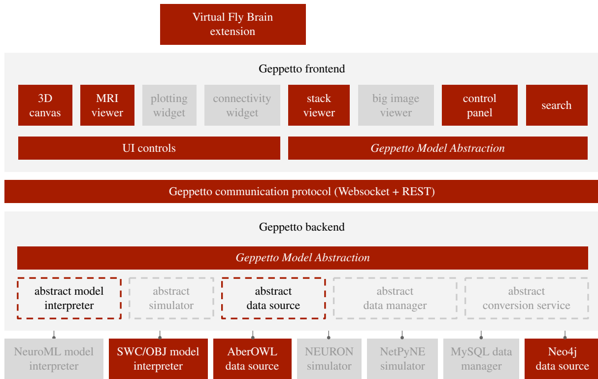
Figure 4. Geppetto VFB configuration. Graphical representation of the components of Geppetto that are used on the VFB application (red). The ones not used are coloured in grey.
