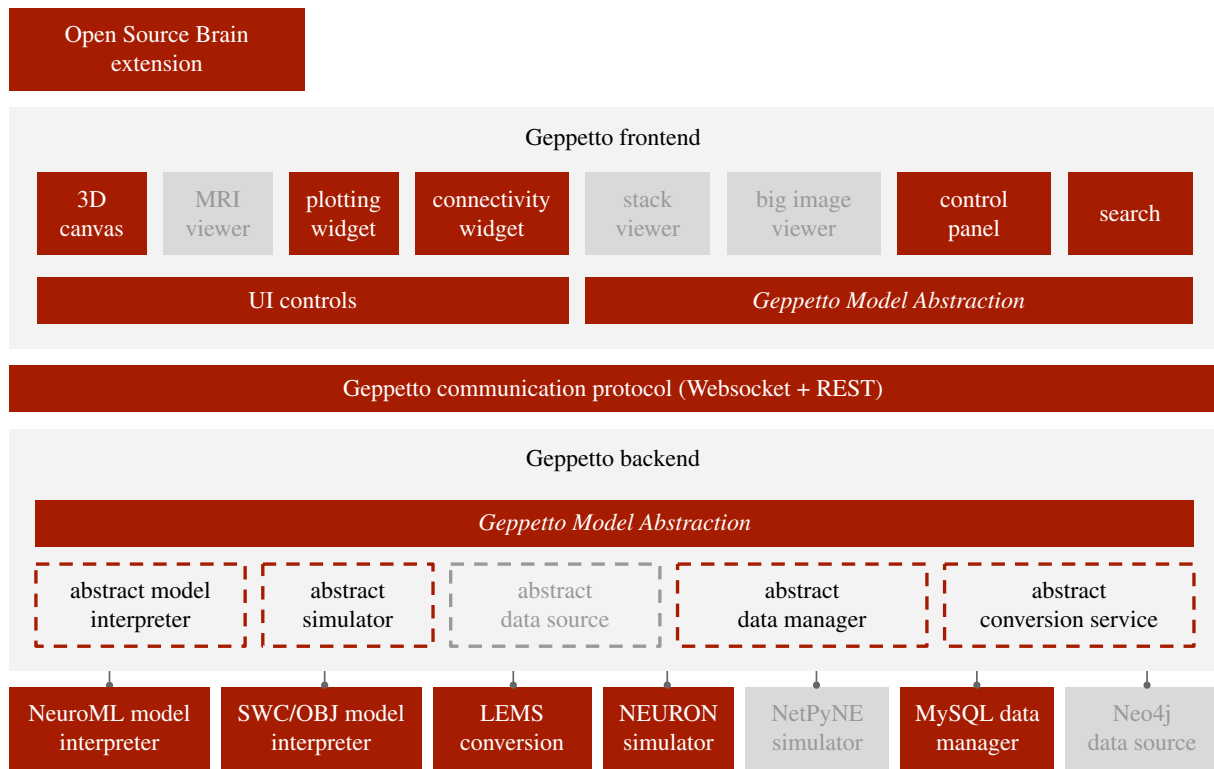
Figure 2. Geppetto OSB configuration. Graphical representation of the components of Geppetto that are used on the OSB application (red). The ones not used are coloured in grey.
