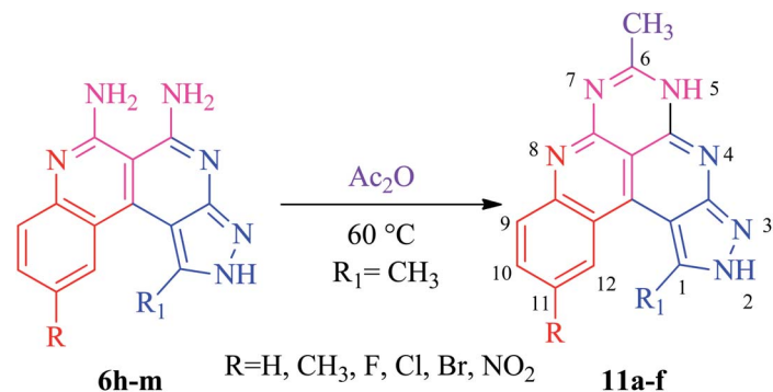
Scheme 6 Synthesis of benzo[ c ]pyrazolo[4,3- f ]pyrimido[4,5,6- ij ][2,7]naphthyridines 11a–f .
