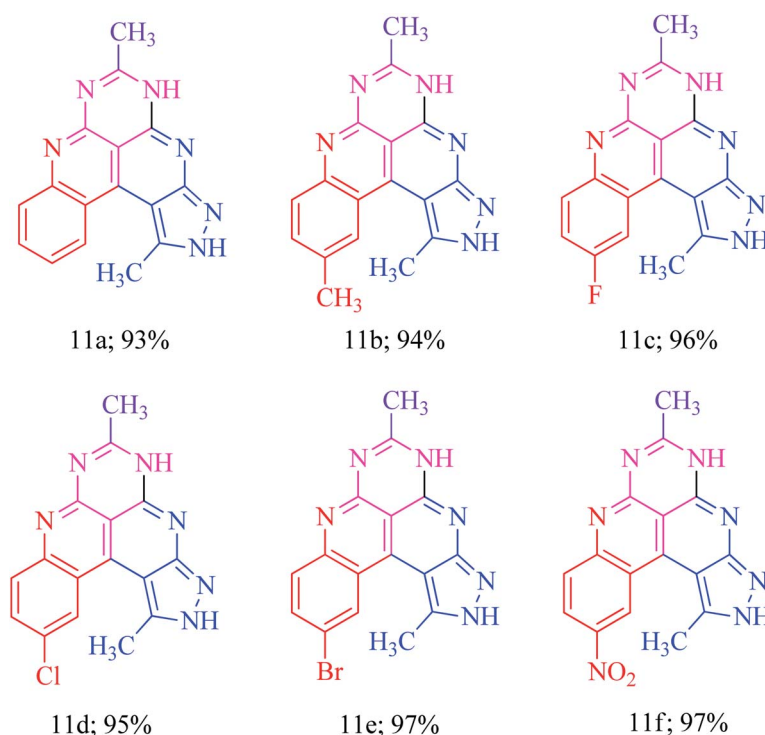
Fig. 3 Substrate scope with different benzo[ c ]pyrazolo[4,3- f ]pyrimido[4,5,6- ij ][2,7]naphthyridines 11a–f . Reaction conditions: benzo[ c ]pyrazolo[2,7]naphthyridines 6h–m (2 mmol), acetic anhydride (6 ml), heat 60 °C (2–3 h).
