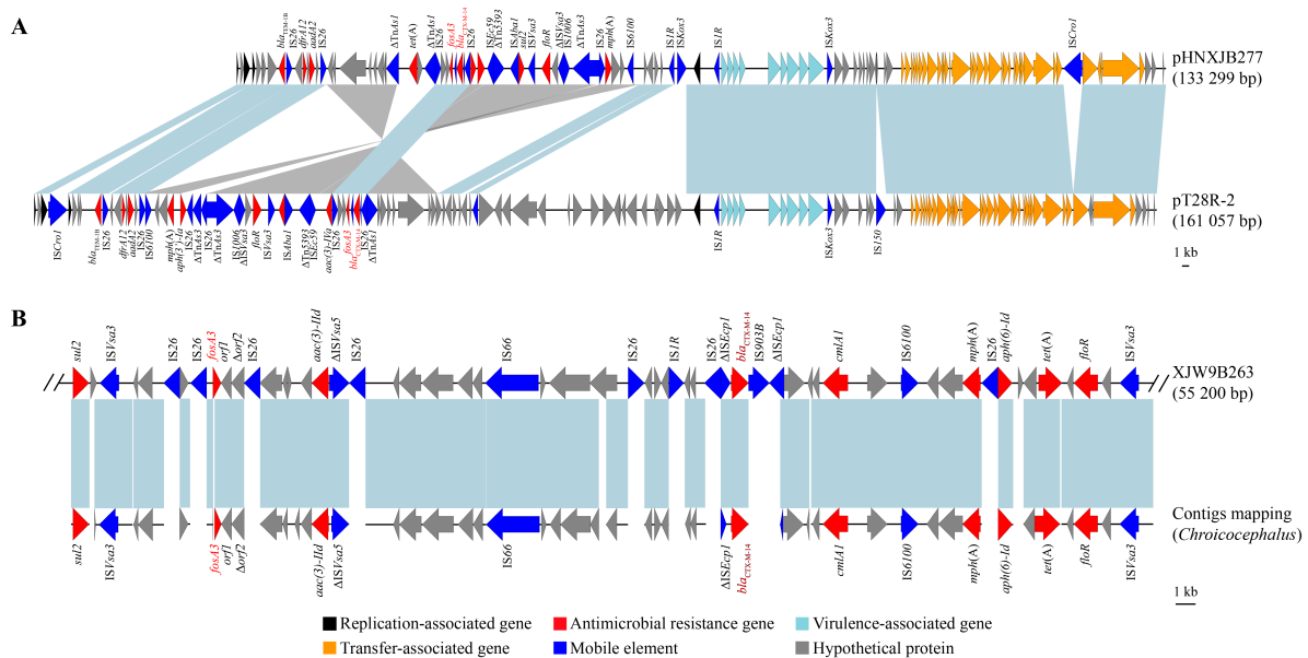
Figure 3 Genetic environment of fosA3 and bla CTX-M-14
