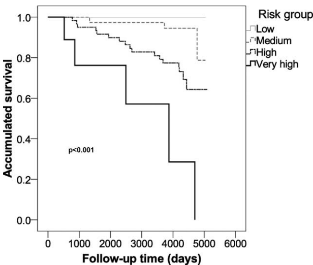
FIGURE 3. Differences between the different risk groups constructed in the validation sample.
