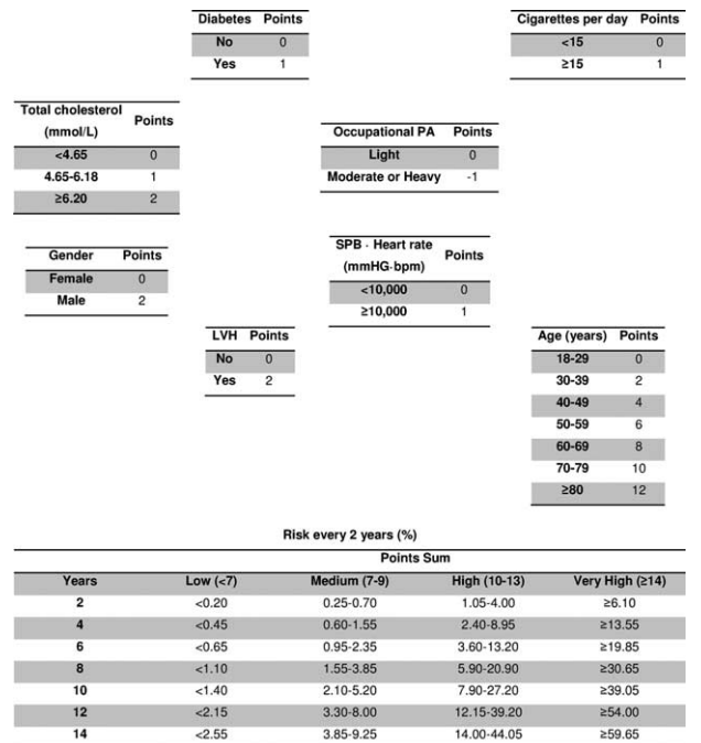
FIGURE 1. Predictive model to determine which patients will suffer a cardiovascular disease within a maximum period of 14 years. Definition of occupational physical activity: light activity: activity associated with sitting at a desk or behind a counter with automated instruments; moderate activity: continuous light physical activity, such as light work in industry or in agriculture out of season; intense activity: heavy work and, at times, energetic (agricultural production, mining, or steel work). If a person was not working, he or she was classified as performing light activity. LVH = left ventricular hypertrophy, PA = physical activity, SBP = systolic blood pressure
