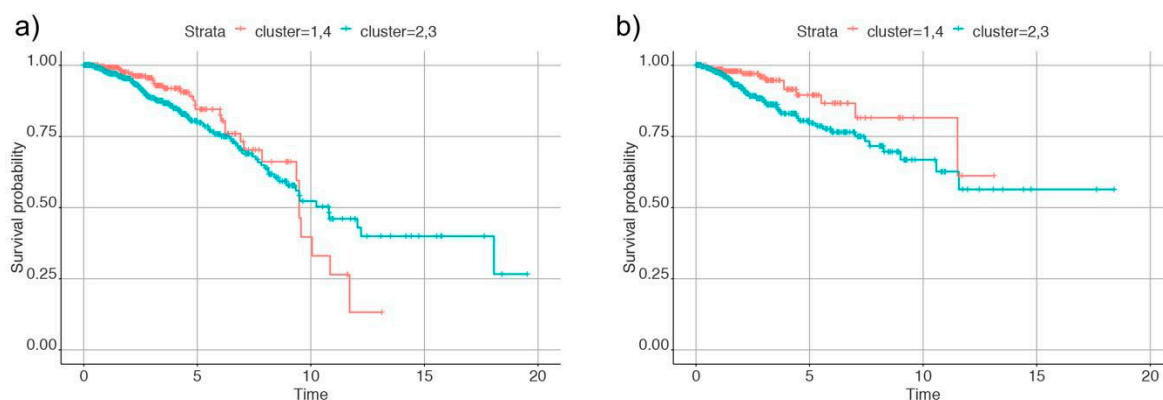
Figure 4. Plots of Kaplan-Meier estimates for (a) overall survival and (b) recurrence of cancer in the individuals. Clusters 1 and 4 are denoted by the red line and clusters 2 and 3 by the blue line.
