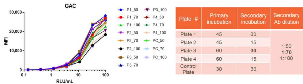
Figure A2. Standard curve optimisation (GAC only shown) with Privigen IVIG serially diluted 3-fold from 1:1000 dilution (nominal concentration 100 RLU/mL) to 1: 1:6,561,000.
