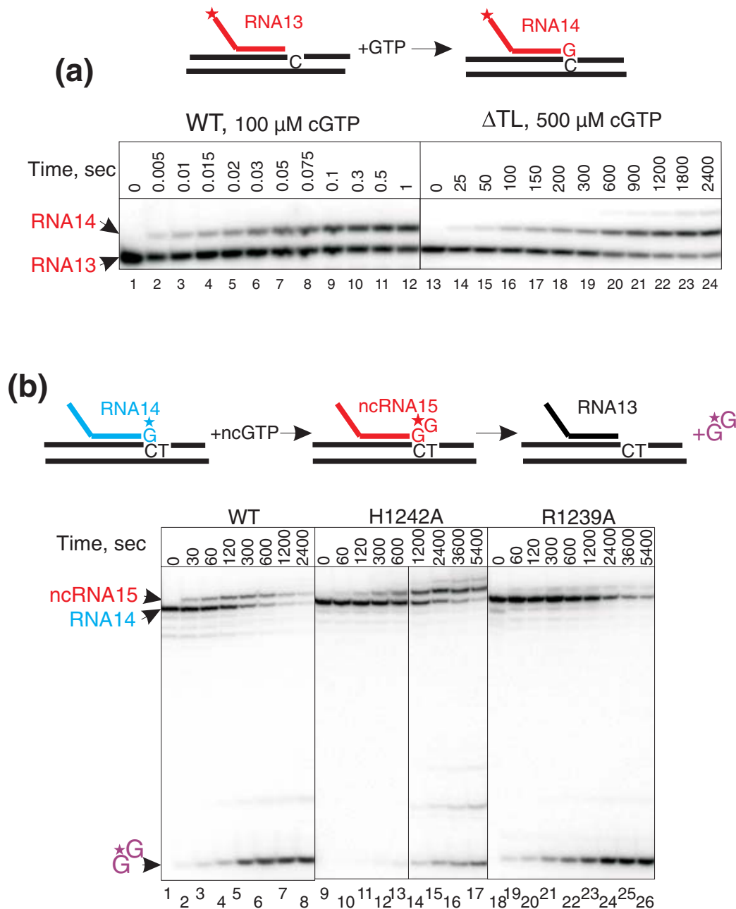
Figure 2 Incorporation and misincorporation by wild-type (WT) and mutant RNA polymerase (RNAPs). (a) Cartoon schematically describes the reaction of cNTP (cGTP) incorporation in EC^{G1} (Additional File 1: Figure S2) with ^{32}P 5'-labelled RNA (asterisk). Elongation complexes are shown with non-template DNA strand below the template strand to reflect their full complementarity (as in Additional File 1: Figure S2). Representative gels of 100 \mu M cGTP incorporation by WT and 500 \mu M cGTP incorporation by \Delta TL in EC^{G1} are shown. The lack of complete extension of transcripts was due to the procedure by which elongation complexes were assembled (see Methods). (b) The intrinsic proofreading reaction accompanies misincorporation. The cartoon above the gel schematically describes the processes going on during ncGTP misincorporation in EC^A (Additional File 1: Figure S2). Elongation complexes are shown with non-template DNA strand below the template strand to reflect their full complementarity (as in Additional File 1: Figure S2). Note that RNAs in elongation complexes were labelled at the 3' end (by incorporation of [^{32}P]GTP ; asterisk), thus allowing monitoring both misincorporation event and removal of the wrong nucleotide via transcript assisted proofreading. Misincorporation of 1 mM ncGTP and proofreading by WT, H1242A and R1239A RNAPs are shown as an example. The cleavage products larger than dinucleotide originate from 2 bp and 3 bp backtracked complexes that undergone further extension after misincorporation. The colours of the RNA products of the reactions are the same as in the scheme of the reaction above the gels. Black vertical line separates lanes originating from the same gel that were brought together.
