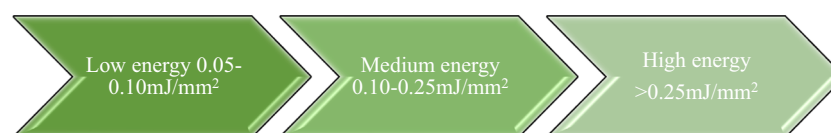
Fig. 3 Energy flux densities (EFD measured in \text{mJ}/\text{mm}^2 ) as low energetic (<0.1 \text{mJ}/\text{mm}^2 ), medium energetic (0.1–0.25 \text{mJ}/\text{mm}^2 ), and high energetic (>0.25 \text{mJ}/\text{mm}^2 )
