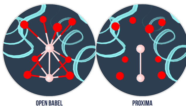
Figure 2. Looking at a difficult case: the potassium channel (PDB ID: 1BL8). (left) Bond perception performed by the Avogadro software 5 (version 1.1.1) (using the OpenBabel library 6 (version 2.3.2)): number of bonds perceived, 2918. (right) Bond perception performed by Proxima: number of bonds perceived, 2897.
