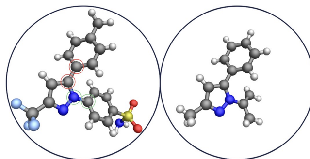
Figure 3. Celecoxib molecule on the left. On the right, the molecular system cut at a distance of four bonds around the red atoms.
