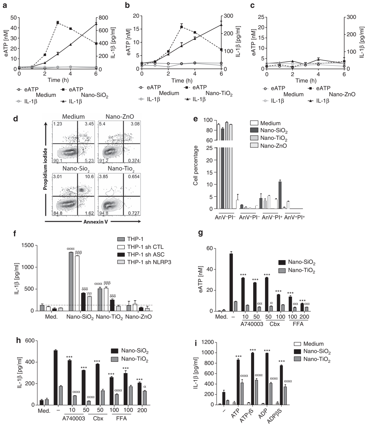
Figure 1 Nano-SiO 2 or nano-TiO 2 particles trigger active ATP release and IL-1β secretion through purinergic signalling and pannexin/connexin hemichannel activity. Nano-SiO 2 (a) or nano-TiO 2 (b) triggered active release of ATP in the supernatant by PMA-primed THP1 that peaks between 3 and 4 h. This ATP release was correlated with a secretion of IL-1β (a,b). Nano-ZnO did not induce ATP release or IL-1β secretion (c). Apoptotic (PI – anV+) and necrotic (PI+ anV –) cell death of primed THP1 was monitored using the AnnexinV/PI staining (d,e). ARL67156 (50 μM) was added to the supernatant during stimulation to limit ATP catabolism (a–c). IL-1β secretion by nano-SiO 2 or nano-TiO 2 was attenuated in THP1 cells stably expressing shRNA directed against ASC (sh ASC) or NLRP3 (sh NLRP3) in comparison with THP1 transfected with lamin-specific shRNA (sh CTL) (f). Nano-ZnO did not induce IL-1β secretion after 4 h of stimulation (f). Specific inhibition of P2X7R by A740003 partially decreased ATP release and IL-1β secretion by PMA-primed THP1 after 4 h nanoparticle stimulation (g,h). Connexin/pannexin channel blocker carbenoxolone (Cbx) and connexin channel blocker flufenamic acid (FFA) reduced both ATP release and IL-1β secretion upon nano-SiO 2 or nano-TiO 2 (g,h). PMA-primed THP1 stimulated for 4 h with 200 μM ATP, ADP or their stable derivatives ATPγS or ADPβS greatly increased IL-1β production in response to nanoparticles, whereas these nucleotides had no effect alone (i). Nanoparticles are at the concentration of 250 μg/ml (a–h) or 125 μg/ml (i). Data are representative of 2–4 independent experiments. Data are mean ± S.D. of triplicates, compared between untreated and nanoparticle-stimulated THP1; ααα, P ≤ 0.001 for THP1, βββ, P ≤ 0.001 for THP1 sh CTL, γγγ, P ≤ 0.001 for THP1 sh ASC, δδδ: P ≤ 0.001 for THP1 sh NLRP3 (f). Data are mean ± S.D. of triplicates, compared between nanoparticle-stimulated THP1 and nanoparticles plus inhibitor or agonist; *** and ααα, P ≤ 0.001 for nano-SiO 2 and nano-TiO 2 stimulated THP1, respectively (g–i)
