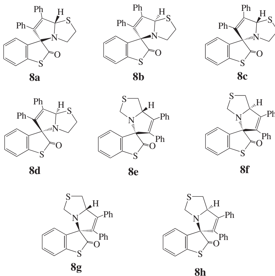
Figure 5 Possible isomers of cycloadduct 8.
