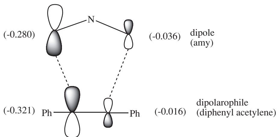
Figure 7 Atomic orbital coefficients and overlapping of dipole(amy) with diphenylacetylene.
