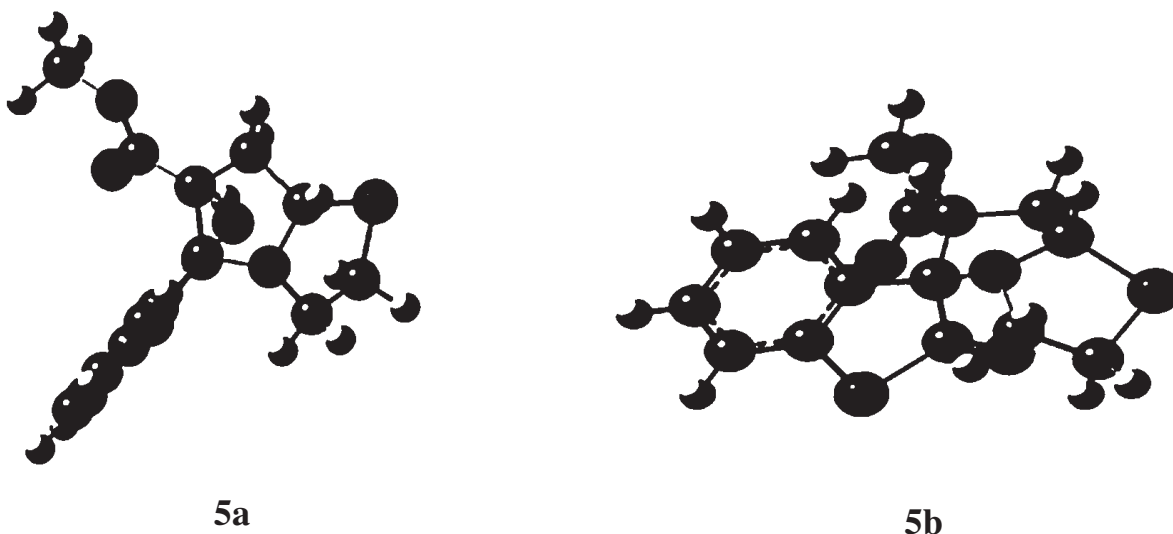
Figure 4 Transition states of cycloadducts 5a and 5b.
