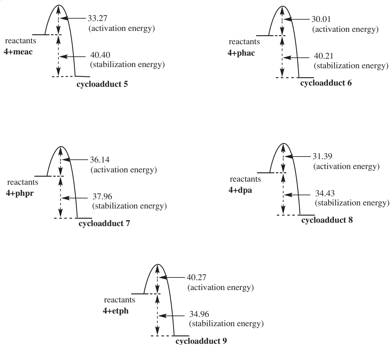
Figure 10 Energy profile diagrams of azabicycloadducts 5-9 (all values in Kcal/mol).
