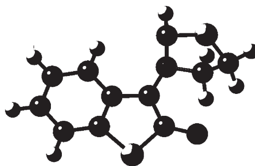
Figure 1 Optimized geometry of amy 4 anti .
