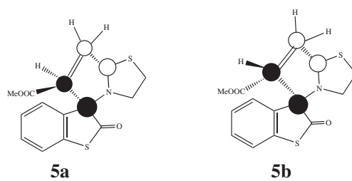
Figure 3 Possible isomers of cycloadduct 5 and its regioselectivity.
