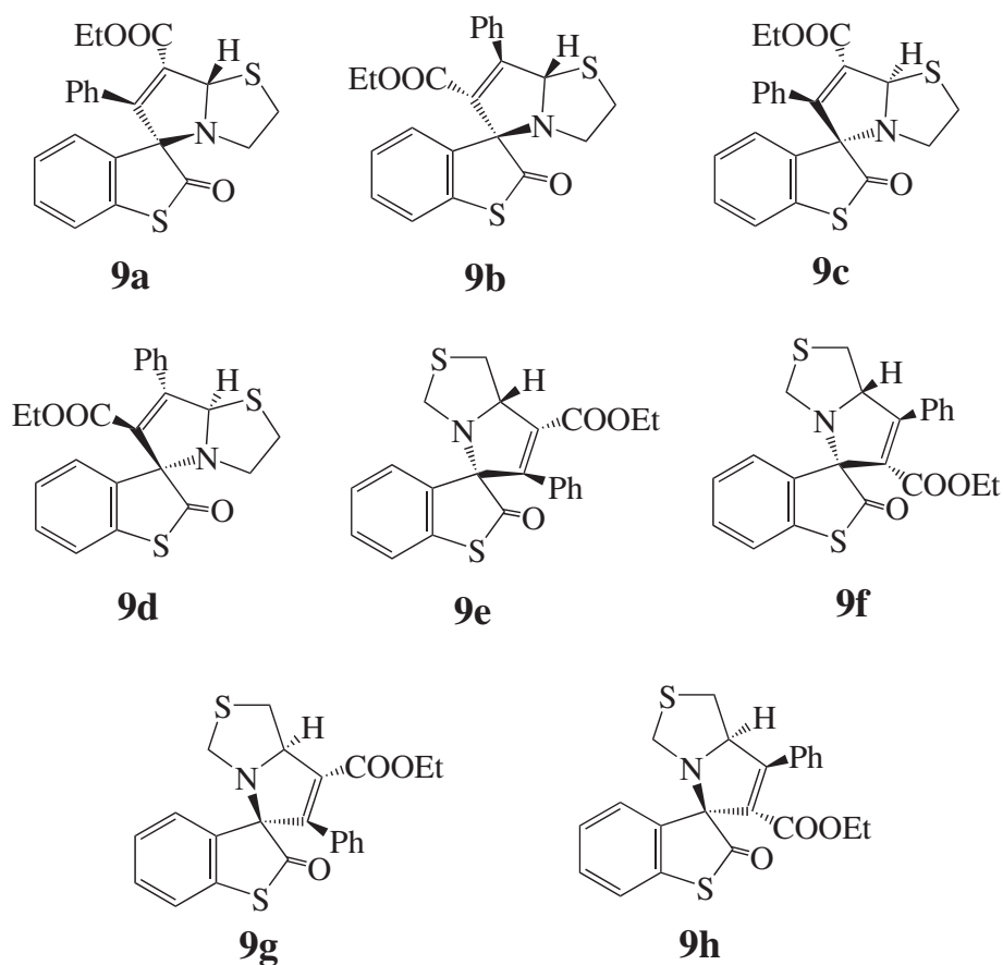
Figure 8 Possible isomers of cycloadduct 9.
