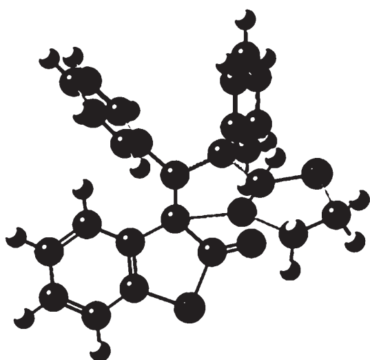
Figure 6 Transition state of diphenylacetylene cycloadduct 8.
