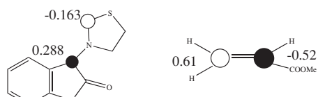
Atomic orbital coefficient of HOMO amy and LUMO methyl acrylate
