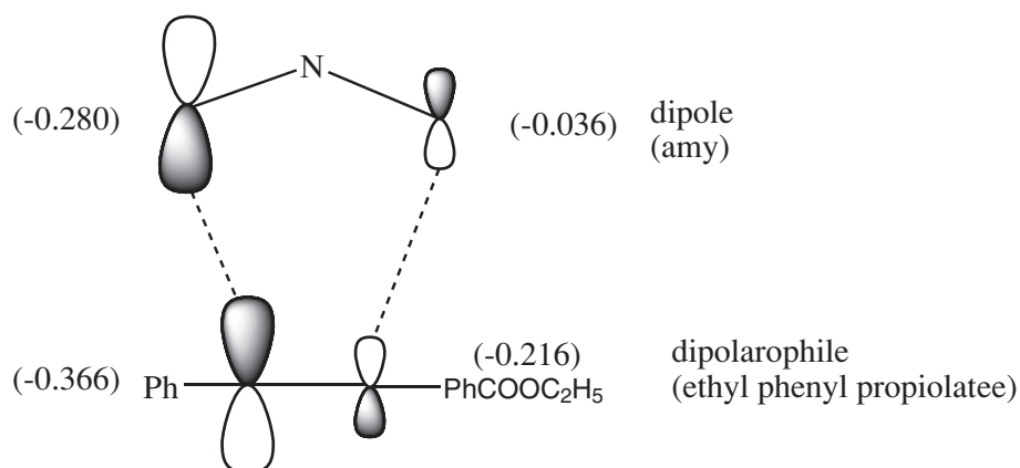
Figure 9 Atomic orbital coefficients and overlapping of amy with ethylphenyl propiolate.
