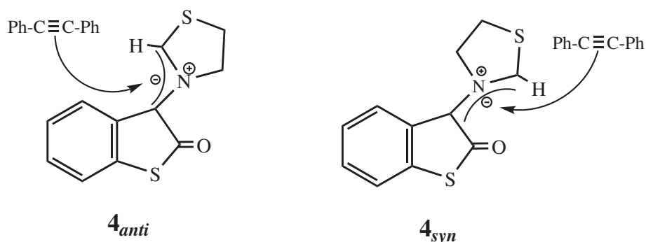
Figure 2 Mode of attack of dipolarophile (diphenylacetylene) on amy 4.
