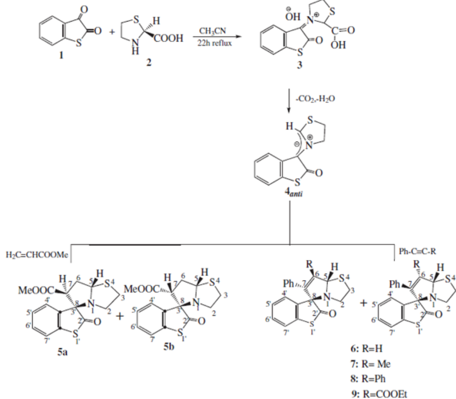
Scheme 1 Reaction of thioisatin with thiazolidine-2-carboxylic acid in presence of different dipolarophiles produced regioisomeric mixtures of cycloadducts.
