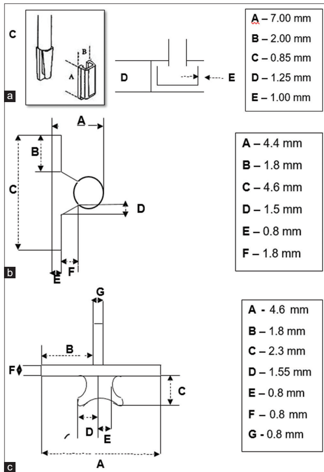
Figure 1: Schematic representation of all attachment designs: (a) PH Conix-PH Intrax, (b) Preci-Vertex standard and Preci-Vertex P (45° inclination), (c) Vario-Soft 3 conical bridge
