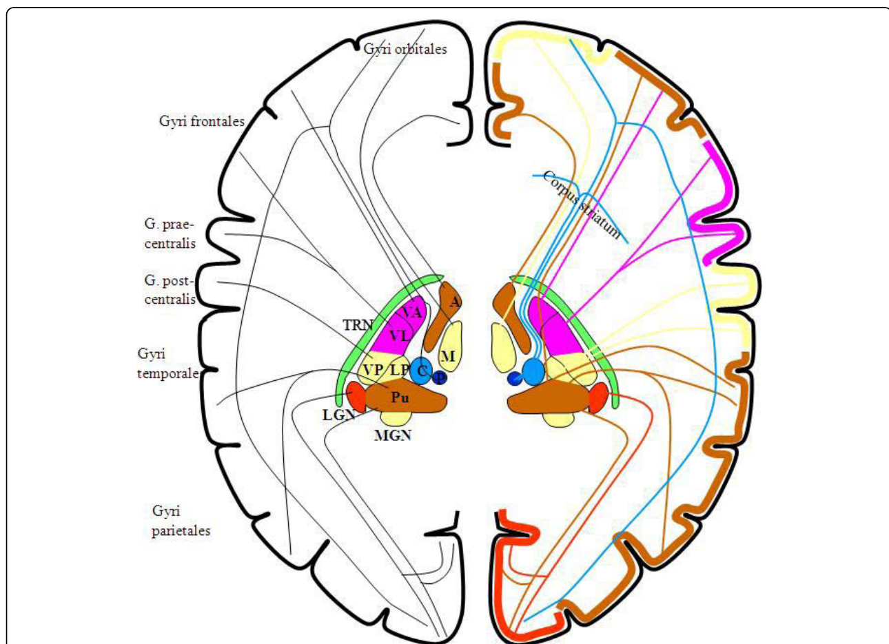
Figure 1 A schematic diagram of the connections between thalamic relay nuclei and their corresponding cortical areas (of the same color) through the thalamic reticular nucleus. Black lines indicate corticothalamic connections, and colored lines indicate thalamocortical connections. A: anterior thalamic nucleus, M: medial thalamic nucleus, VA: ventral anterior nucleus, VL: ventral lateral nucleus, VP: ventral posterior nucleus, LP: lateral posterior nucleus, Pu: pulvinar, C: centromedial nucleus, P: parafascicular nucleus, LGN: lateral geniculate nucleus, MGN: medial geniculate nucleus, TRN: thalamic reticular nucleus (courtesy of Wolfgang Klimesch, with permission).
